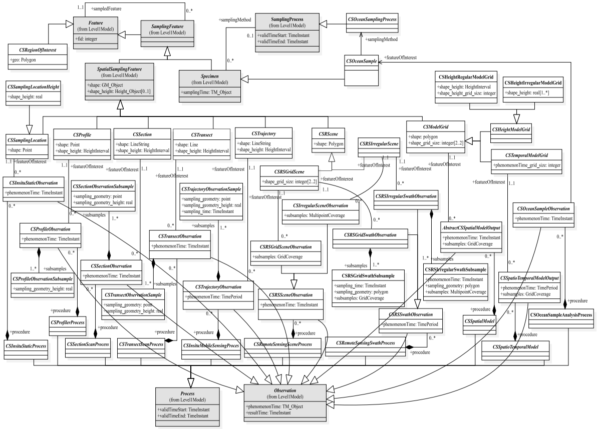
Fig. 3. Level 3 data model for climate science.
