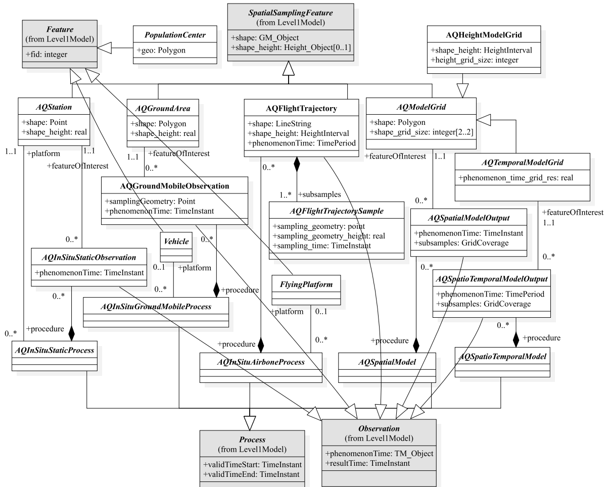
Fig. 13. Level 3 data model for air quality.
