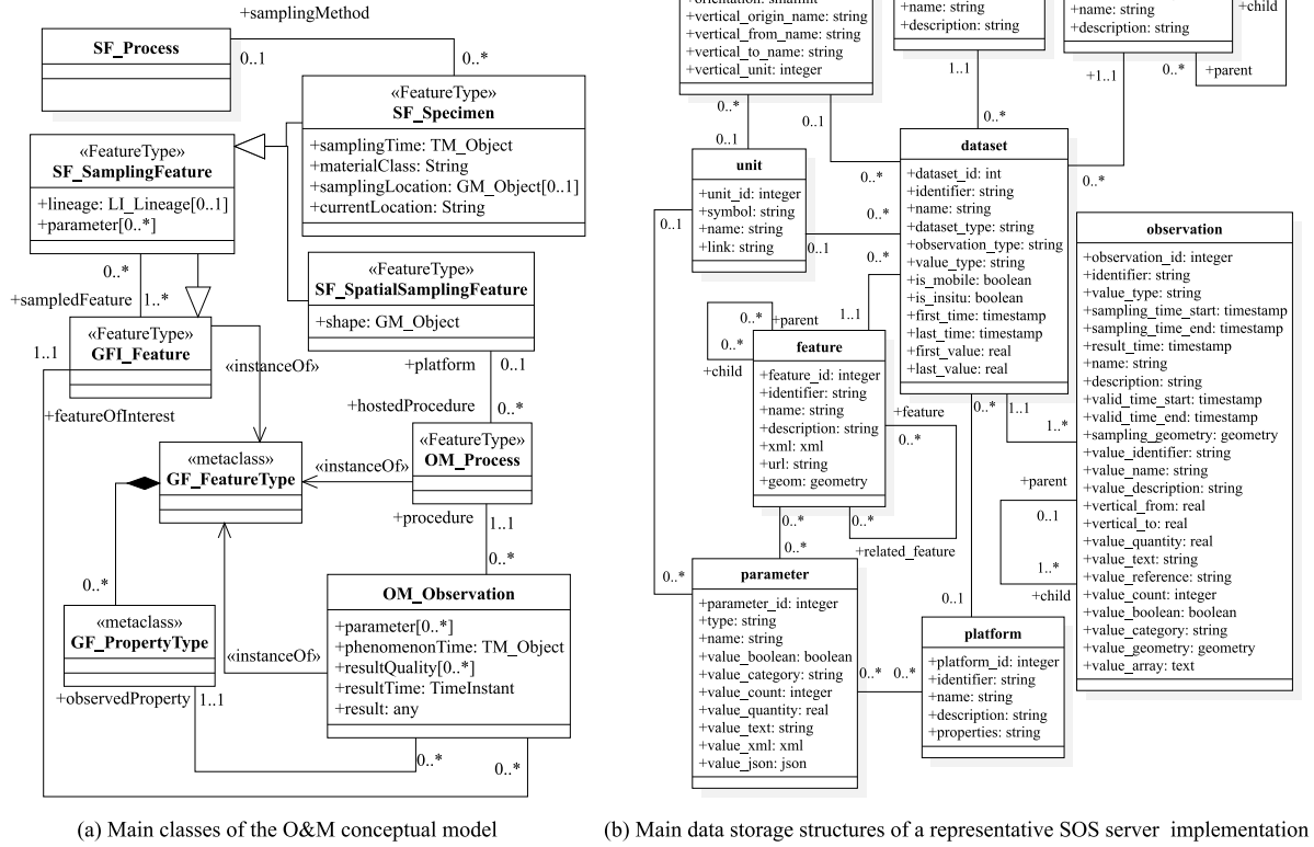
Fig. 1. Illustration of a general purpose data storage model based on OGc O&M.
