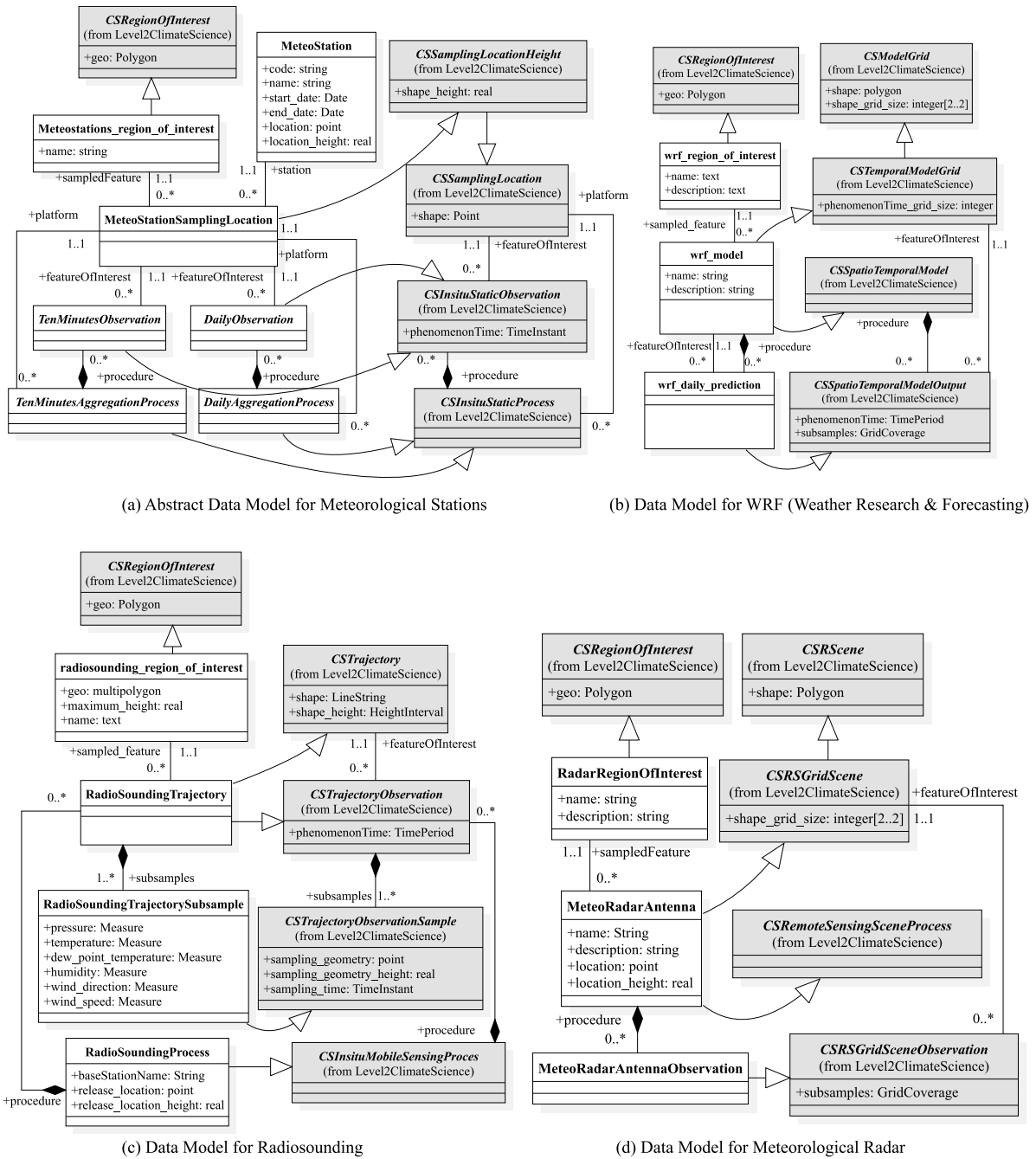
Fig. 4. Level 4 data models for meteorological data in MeteoGalicia.
