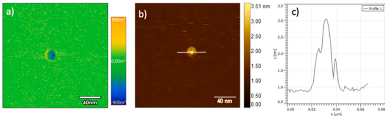
Fig. 2. a) MFM phase shift image of a single nanoparticle of the FeCo exc alloy and b) its corresponding topographical image; c) nanoparticle profile along the white line marked in b).
