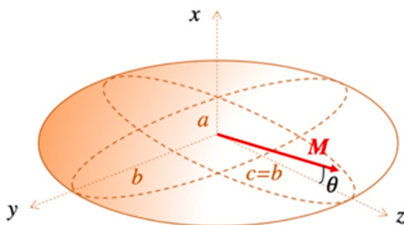
Fig. 12. Graphic representation of an \text{Fe}_x\text{Co}_{1-x} alloy single nanoparticle as an oblate spheroid, with its magnetization M lying in the xz plane.
