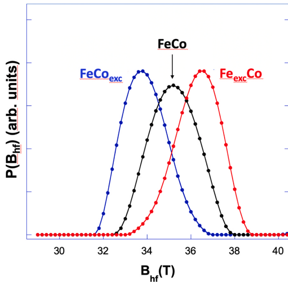
Fig. 11. Room temperature hyperfine field distribution obtained from Mössbauer spectra of the \text{Fe}_x\text{Co}_{1-x} NPs studied in this work.
