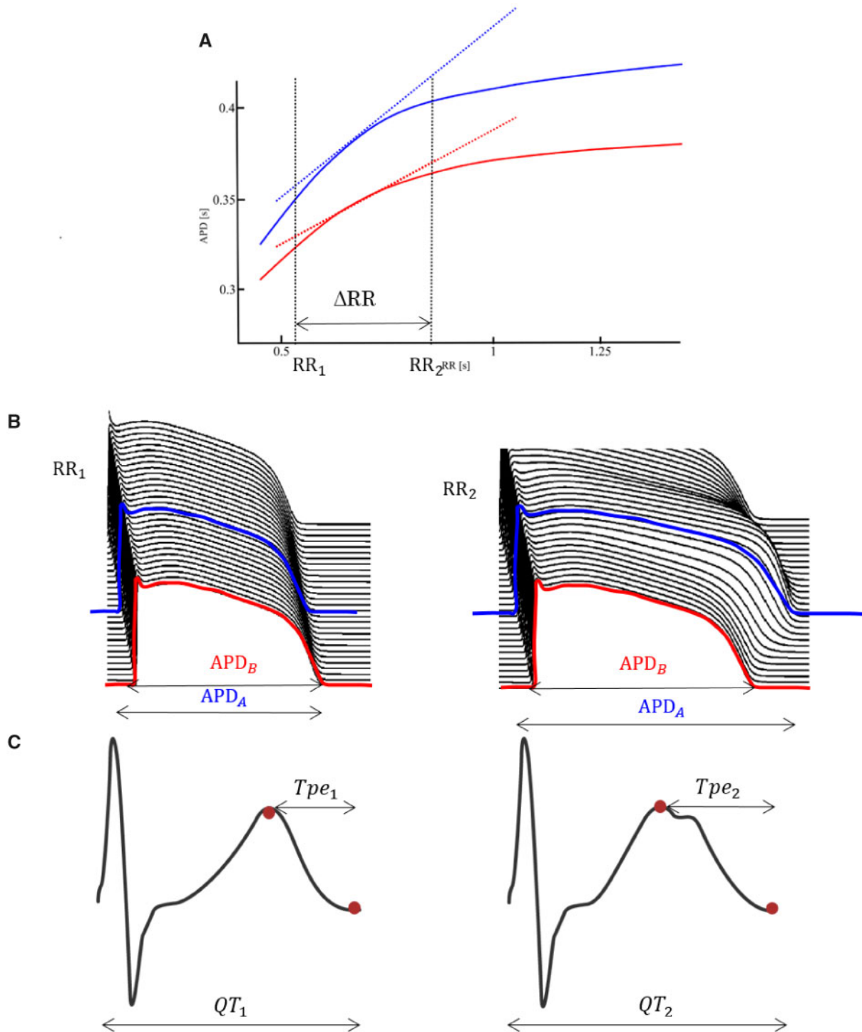
Figure 1. Electrical Restitution. (A) Two APD restitution curves, depicting the APD as a response to the preceding RR interval, of two cardiomyocytes, A (blue) and B (red). (B) The slope of the APD restitution curve measures the change in APD with respect to a change in RR, and high values have been associated with increased arrhythmic predisposition. These changes in the APD are reflected on the ECG signal, as shown in (C).
