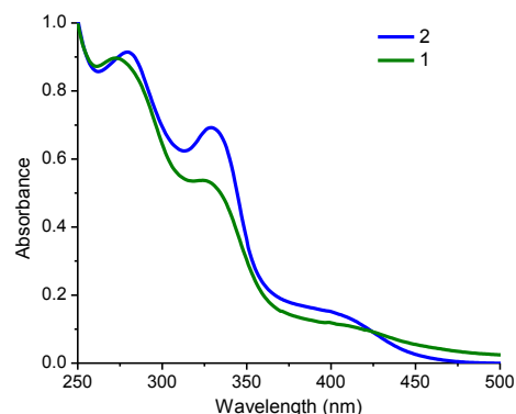
Fig. 4 UV-absorption spectra of complexes 1 and 2 recorded in degassed dichloromethane at 298 K.
