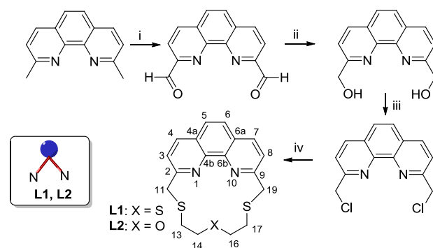
Scheme 1 Depiction of the synthesis of ligands L1 and L2 with the numbering scheme adopted for 1 H and 13 C NMR assignments. (i): SeO 2 , dioxane, reflux; 4h; (ii) NaBH 4 , ethanol, reflux 2h; (iii) SOCl 2 , r.t., 8h; (iv) (HSCH 2 CH 2 ) 2 S ( L1 ) or (HSCH 2 CH 2 ) 2 O ( L2 ), Cs 2 CO 3 , dimethylformamide (dmf), 55 °C.
