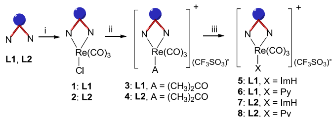
Scheme 2 Depiction of the synthesis of species 1-8 (i): [ReCl(CO) 3 ], Toluene, reflux 1h; (ii) [Ag(CF 3 SO 3 )], acetone, r.t. 12h; (iii) Py/ImH, THF/acetone, r.t., 1d/4d.
