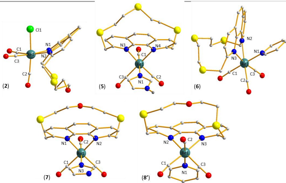
Fig. 2 Molecular structure of complex 2 and complex cations in 5 , 6 , 7 and 8' respectively. The most relevant bond lengths (Å) and angles (deg): Complex 2 : Re(1)–C(1) = 1.903(3), Re(1)–C(2) = 1.903(3), Re(1)–C(3) = 1.912(3), Re(1)–N(1) = 2.206(3), Re(1)–N(2) = 2.237(3), Re(1)–Cl(1) = 2.4963(10); N(1)–Re(1)–N(2) = 74.01(10), Cl(1)–Re(1)–C(2) = 174.85(9); Complex 5 : Re(1)–C(1) = 1.915(4), Re(1)–C(2) = 1.905(3), Re(1)–C(3) = 1.925(4), Re(1)–N(1) = 2.187(3), Re(1)–N(3) = 2.214(3), Re(1)–N(4) = 2.195(3); N(4)–Re(1)–N(3) = 74.35(10), C(1)–Re(1)–N(1) = 177.04(12); Complex 6 : Re(1)–C(1) = 1.935(13), Re(1)–C(2) = 1.943(12), Re(1)–C(3) = 1.924(13), Re(1)–N(1) = 2.209(10), Re(1)–N(2) = 2.219(9), Re(1)–N(3) = 2.206(9); N(3)–Re(1)–N(2) = 74.9(3), C(1)–Re(1)–N(1) = 177.6(4); Complex 7 : Re(1)–C(1) = 1.924(4), Re(1)–C(2) = 1.920(2), Re(1)–C(3) = 1.913(4), Re(1)–N(1) = 2.204(3), Re(1)–N(2) = 2.199(3), Re(1)–N(3) = 2.1803(19); N(2)–Re(1)–N(1) = 74.62(10), C(2)–Re(1)–N(3) = 177.61(12); Complex 8' : Re(1)–C(1) = 1.919(5), Re(1)–C(2) = 1.920(5), Re(1)–C(3) = 1.899(4), Re(1)–N(1) = 2.215(4), Re(1)–N(2) = 2.220(4), Re(1)–N(3) = 2.209(3); N(3)–Re(1)–N(2) = 74.58(13), C(2)–Re(1)–N(1) = 174.74(14).
