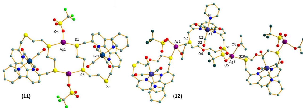
Fig. 3 Molecular structure of dimeric and polymeric assemblies in compounds 11 and 12 . The most relevant bond lengths (Å) and angles (deg): Complex 11 : Re(1)–C(1) = 1.921(15), Re(1)–C(2) = 1.906(13), Re(1)–C(3) = 1.918(17), Re(1)–N(1) = 2.214(12), Re(1)–N(2) = 2.215(10), Re(1)–N(3) = 2.214(13), Ag(1)–O(4) = 2.365(18), Ag(1)–S(2) = 2.470(4), Ag(1)–S(1) = 2.522(4); N(2)–Re(1)–N(3) = 74.2(4), C(1)–Re(1)–N(2) = 169.9(5), O(4)–Ag(1)–S(2) = 106.4(5), O(4)–Ag(1)–S(1) = 86.3(5), S(1)–Ag(1)–S(2) = 148.81(14); Complex 12 : Re(1)–C(1) = 1.940(11), Re(1)–C(2) = 1.874(10), Re(1)–C(3) = 1.893(12), Re(1)–N(1) = 2.225(8), Re(1)–N(2) = 2.212(10), Re(1)–N(3) = 2.215(9), Ag(1)–S(2) = 2.656(5), Ag(1)–S(1) = 2.502(3); N(2)–Re(1)–N(3) = 75.4(3), C(2)–Re(1)–N(1) = 176.7(4), S(1)–Ag(1)–S(2)#2 = 129.30(14) (#2 = x, –y, z+1/2).
