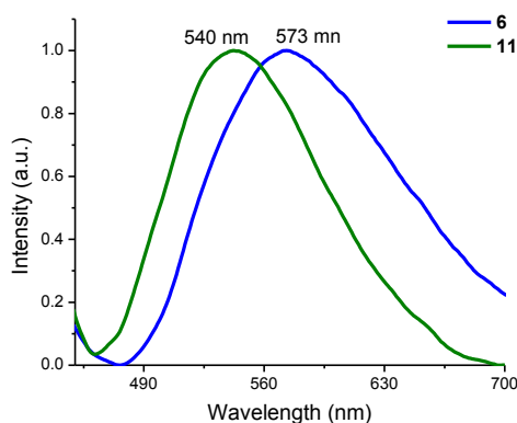
Fig. 5 Emission spectra of complexes 6 and 11 recorded in degassed dichloromethane at 298 K.
