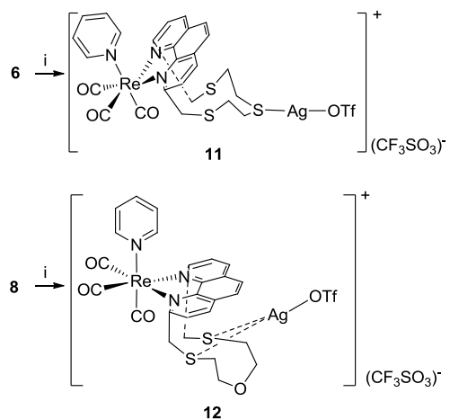
Scheme 4 Depiction of the synthesis of complexes 11 and 12 with the proposed structure in solution (i): [\text{Ag}(\text{CF}_3\text{SO}_3)] , acetone, r.t., 1-3d.
