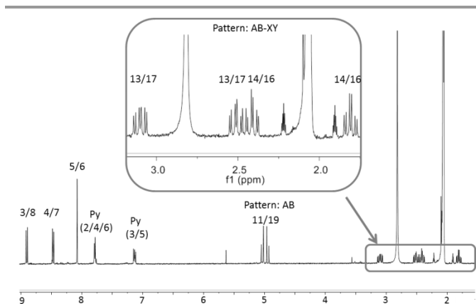
Fig. 1 ^1\text{H} -NMR spectrum of complex 11 .
