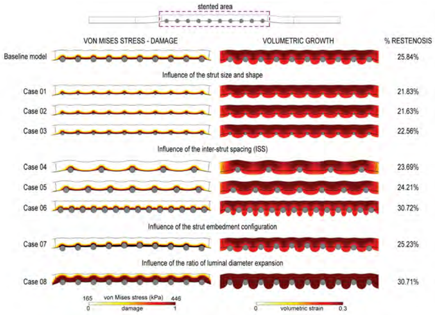
Fig. 12: The impact of different geometric configurations (Table 2) on Von Mises stress distribution and volumetric growth after 300 days.
