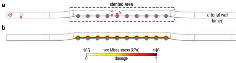
Fig. 5: (a) Deformed computational geometry and (b) von Mises stress distribution and corresponding quantification of the initial damage in the arterial wall. Points A and C are located close to a central stent strut in the media and in the denuded SES between struts, respectively. Points B and D are situated far away from the stented area in the media and SES, respectively.
