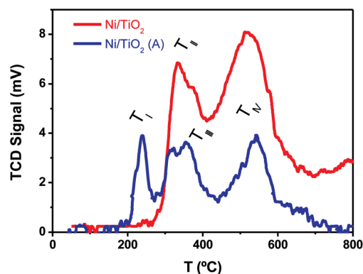
Fig. 3 TPR plots of \text{TiO}_2 before and after Ni photodeposition in \text{MeOH}/\text{H}_2\text{O} , as prepared ( \text{Ni}/\text{TiO}_2 ), and after thermal activation at 400^\circ\text{C} in a 10\%-\text{H}_2 atmosphere ( \text{Ni}/\text{TiO}_2\text{-A} ).
