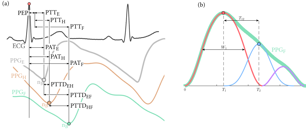
Fig. 1. Illustration of PAT, PTTD, and PDA definitions. (a) The ECG, earlobe (PPG E ), forehead (PPG H ), and finger (PPG F ) PPG signals with the corresponding definitions of PAT E (earlobe), PAT H (head), PAT F (finger), and PTTD EH (earlobe-head), PTTD EF (earlobe-finger), PTTD HF (head-finger). Pulse Transit Time (PTT) refers to the time interval from the end of the Pre-Ejection Period (PEP) following a heartbeat to the arrival of the pulse wave at a peripheral site. The PEP interval shown is merely illustrative. (b) The characteristics of a PPG pulse waveform at the fingertip with PDA are shown. The PPG waveform is depicted in green, while the first, second, and third waves are indicated by red, blue, and magenta colors, respectively. The image emphasizes the morphological features based on the width ( W_1 ) and the time interval ( T_{12} ) for the first and second inner waves.
