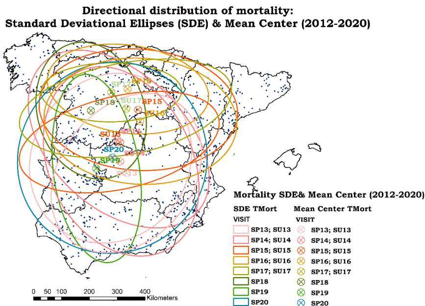
Figure 1: Directional distribution & Mean center of winter (SP) and spring (SU) mortality (2012-2020).
