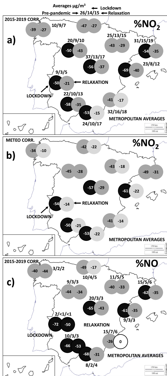
Fig. 5. a) Into circles: averaged percentage change of NO 2 compared to the 2015–2019 averages; over or below circles: average concentrations (in µg/m 3 ) during the pre-pandemic/lockdown/relaxation periods. b) Idem but circles indicate meteorology corrected reductions. c) Idem for NO concentrations and averaged percentage change of NO compared to the 2015–2019 averages.
