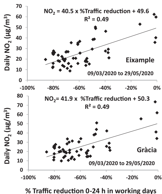
Fig. 7. Cross correlation plots and regression equations for the percentage of reductions of traffic daily counts and daily NO 2 ambient concentrations recorded at two traffic air quality monitoring stations of Barcelona (Eixample and Gràcia) from before (09/03/2020) to the end (29/05/2020) of the lockdown.
