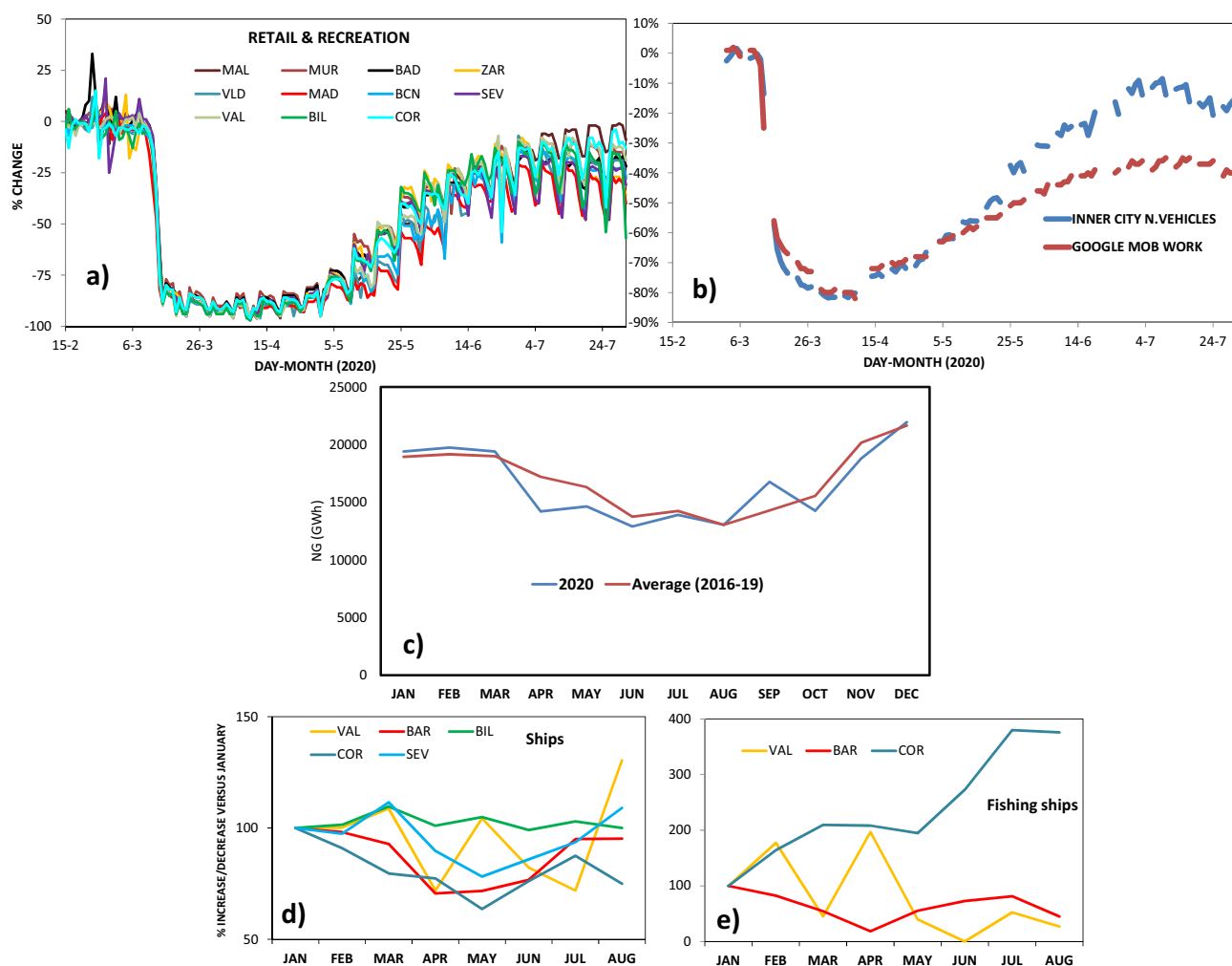
Fig. 3. a) Human mobility changes (%; Google LLC, 2020) from average baseline (calculated with data from 03/01 to 06/02/2020) in Málaga (MAL), Murcia (MUR), Badajoz (BAD), Zaragoza (ZAR), Valladolid (VLD), Madrid (MAD), Barcelona (BCN), Sevilla (SEV), Valencia (VAL), Bilbao (BIL) and A Coruña (COR) (Spain), before, during and after the lockdown imposed by COVID-19. b) Comparison of the relative variation of the week day circulating vehicles (provided by Barcelona City Council) and the ones for work-place Google Mobility. c) Monthly natural gas consumed by the industry in Spain (excluding power generation, in GWh) in 2020 compared with 2016–2019 averages (calculated with data obtained from Enagas, 2021 and Cores, 2021). d) Relative changes (%; Puertos del Estado, 2020) of the monthly number of ships and e) fishing ships in harbors from the study cities.
