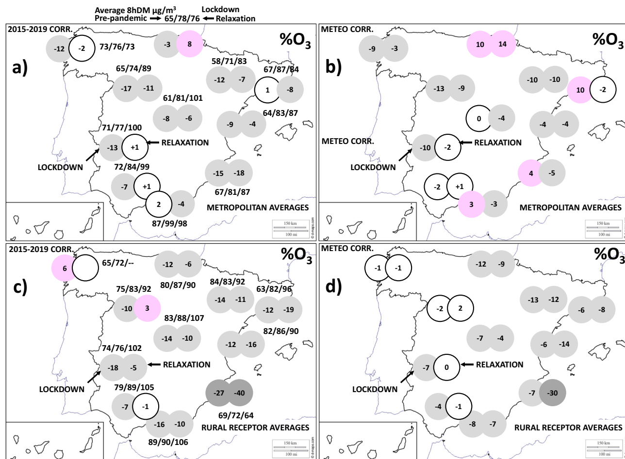
Fig. 10. a) Into circles: averaged percentage change of O 3 8hDM in metropolitan areas compared to the 2015–2019 averages in metropolitan areas; over or below circles: average concentrations (in \mu\text{g}/\text{m}^3 ) during the pre-pandemic/lockdown/relaxation periods. b) Idem but circles indicate meteorology corrected reductions in metropolitan areas. c) Idem but circles indicate, for the receptor areas, the reductions compared to the 2015–2019 averages; over or below circles: average concentrations (in \mu\text{g}/\text{m}^3 ) during the pre-pandemic/lockdown/relaxation periods for the receptors. d) Idem but circles indicate meteorology corrected reductions in receptor areas.
