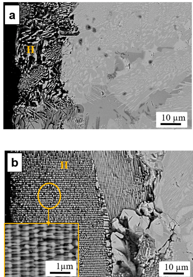
Fig. 3. SEM micrographs of a directionally solidified rod grown at 15 mm/h and after soaking in SBF solution for 3 days: (a) transverse cross section of the rod, (b) transformed Akermanite/TCP region after immersion in SBF in longitudinal cross section. An area with higher magnification is shown in the insert.
