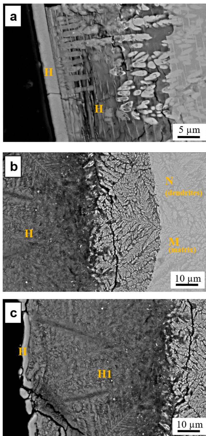
Fig. 5. SEM micrographs of a directionally solidified rod grown at 100 mm/h after soaking in SBF solution for 1 week: (a) transversal cross section (b) longitudinal cross section. Right: unaffected part of the sample, middle: area where the monticellite has transformed and dendrites of Nurse's A phase remain unaltered, left: both phases have transformed to HA (c) longitudinal cross section zone: formation of a HA layer on the surface in contact with SBF.
