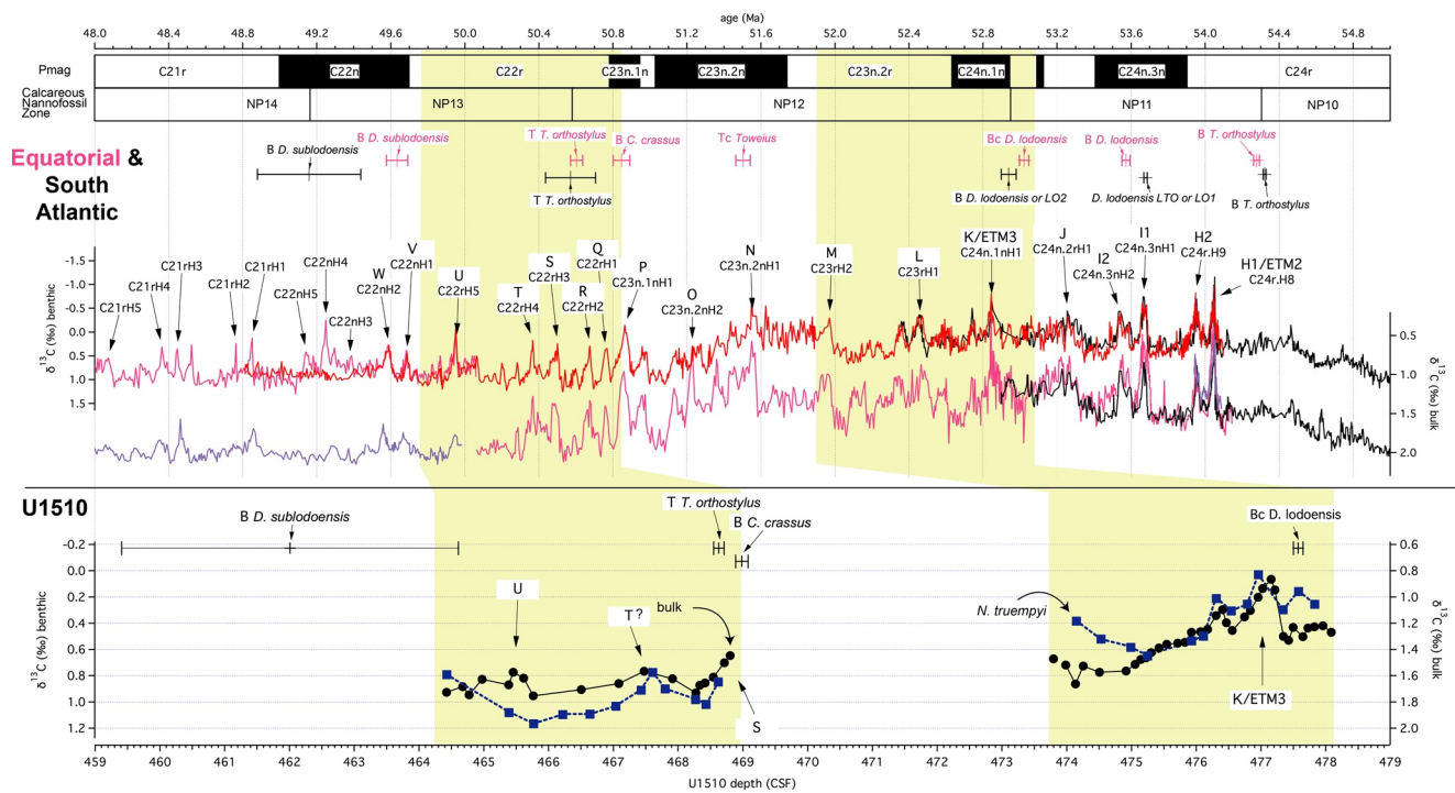
Figure 5. Correlation of Site U1510 with the composite isotope suite and the bio-magnetostratigraphic framework available from the South Atlantic. Top panel: South Atlantic International Ocean Discovery Program Sites 1258 (pink), 1262 (black), 1263 (red) and 1265 (blue) bio- and magnetostratigraphic data as well as benthic and bulk stable isotopes on astrochronology (from Westerhold et al., 2017). Lower panel: U1510 calcareous nannofossil events, benthic and bulk stable isotopes (all this study) and \delta^{13}C ratio (Sutherland, Dickens, Blum, Agnini, Alegret Bhattacharya, et al., 2019) against depth. Yellow intervals show our interpretation of the range cored in U1510 based on calcareous nannofossil assemblages, stable isotopes and an average sedimentation rate.
