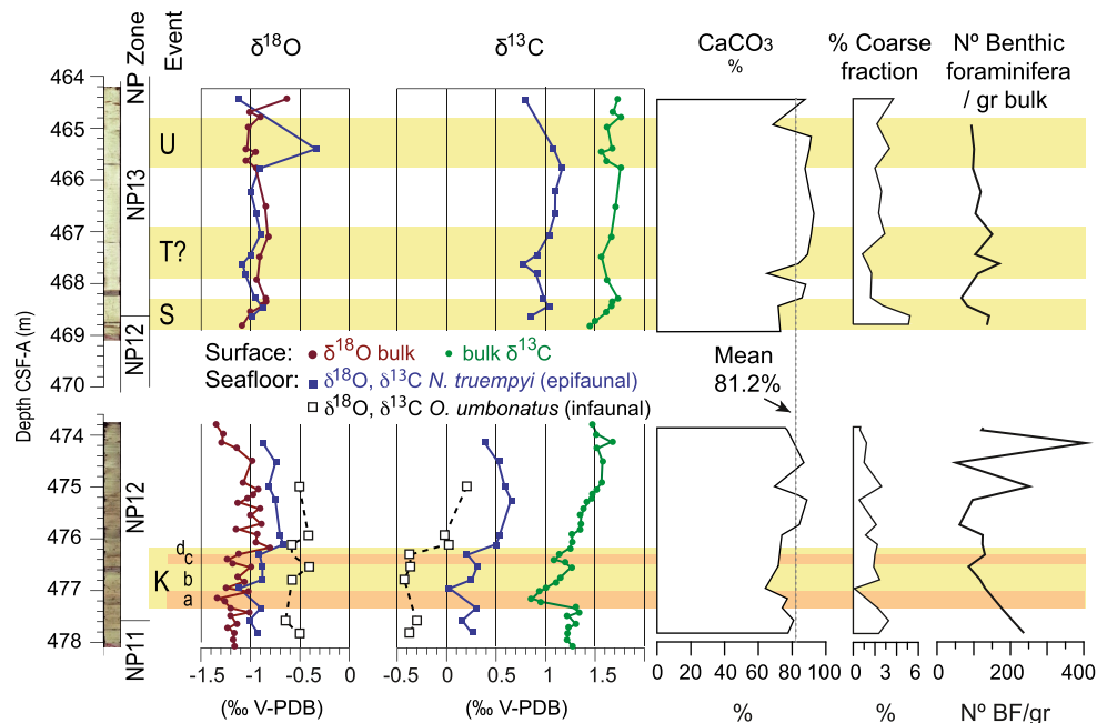
Figure 3. Stable isotopes, % \text{CaCO}_3 , relative abundance of coarse fraction (CF) and number of benthic foraminifera per gram at Site U1510, plotted against depth.
