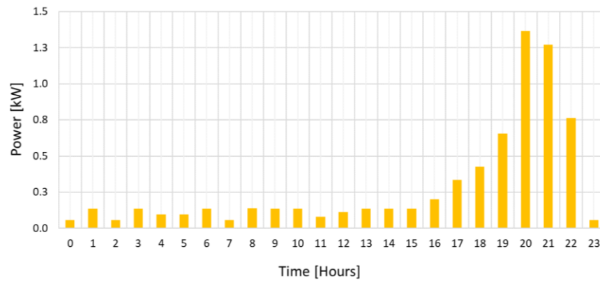
Figure 7. Daily electrical power demand
