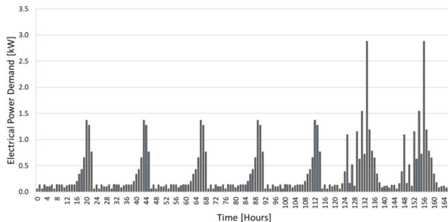
Figure 9. Weekly electrical power demand
