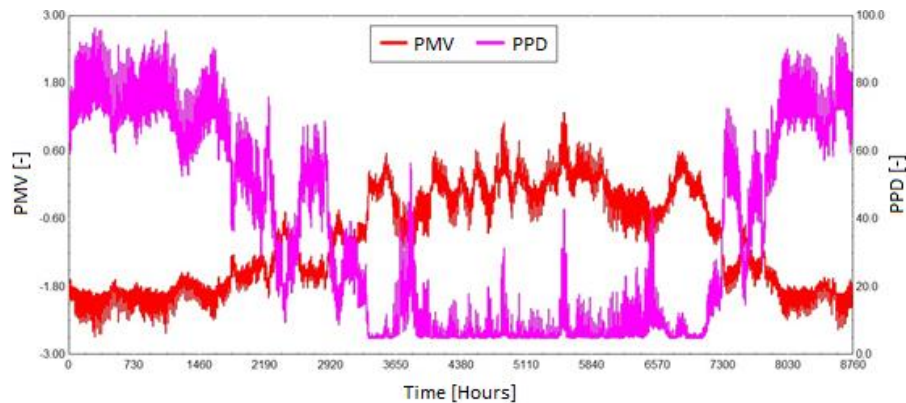
Figure 15. Thermal comfort analysis with temperature control
