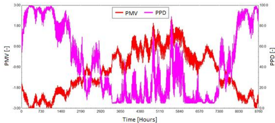
Figure 14. Thermal comfort analysis without temperature control
