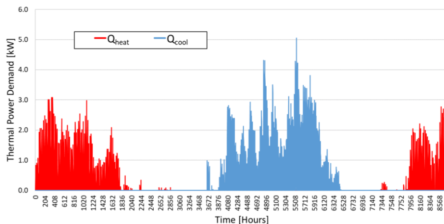
Figure 10. Yearly heating and cooling demand
