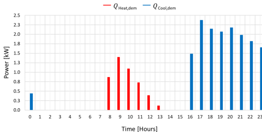
Figure 6. Daily heating and cooling demand
