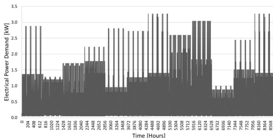
Figure 11. Yearly electricity demand
