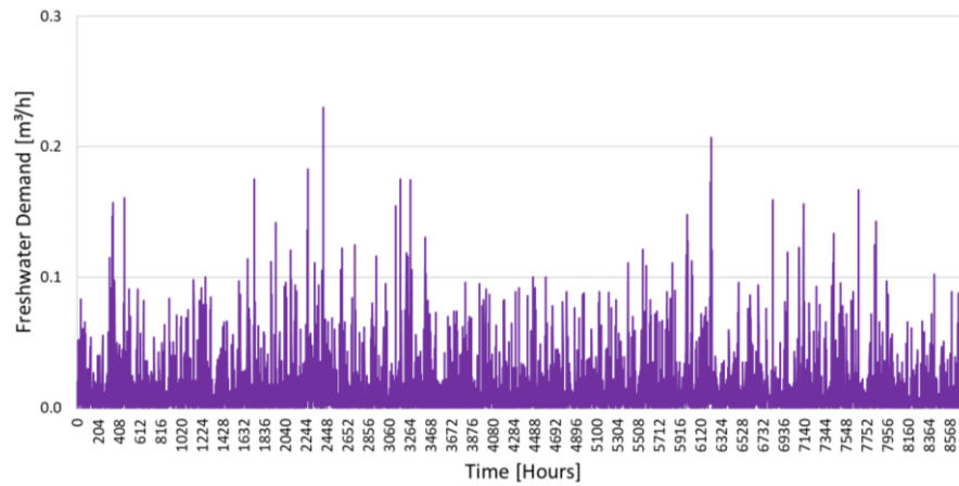
Figure 13. Yearly freshwater demand
