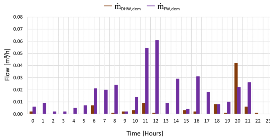
Figure 8. Daily DHW and freshwater flow rate demand
