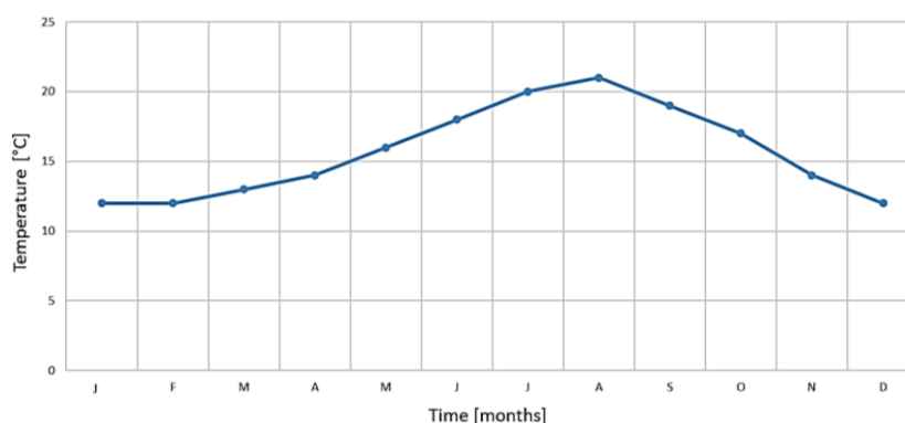
Figure 5. Monthly mean aqueduct water temperature of Almería
