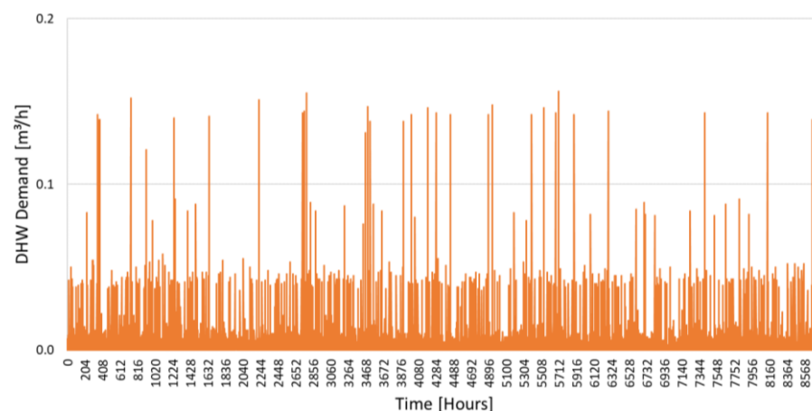
Figure 12. Yearly DHW demand
