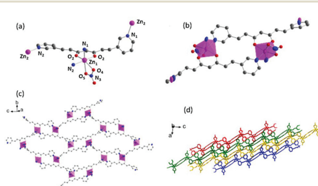
Fig. 4 Crystal structure of 2 : (a) Representation of the coordination sphere of a Zn II centre and the coordination mode of 3pyCCMoid; (b) picture of the smallest loop in the layer; (c) single 2D layer; (d) framework consisting of packed 2D layers (each layer represented by a different colour). Colour legend: Zn, pink; C, grey; O, red; N, blue; H atoms are omitted for clarity.
