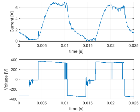
FIGURE 13. Voltage and current for the benchmark SRM at base speed and rated torque.
