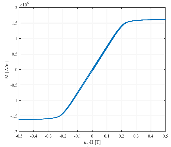
FIGURE 6. Magnetisation (BM) curve of additively manufactured Fe-5%w.t.Si sample.
