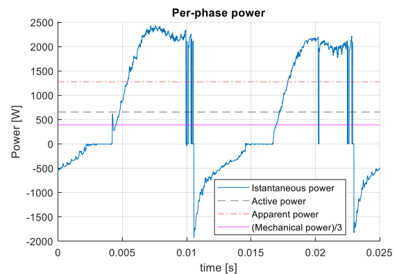
FIGURE 14. Instantaneous power for the benchmark SRM at base speed and rated torque.
