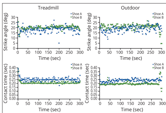
Figure 7.—Strike angle and ground contact time while running on a treadmill and outdoors comparing two different commercially available running shoes.
