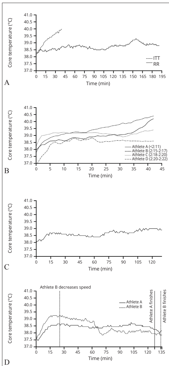
Figure 1.—Core temperature monitoring during the Individual Time Trial (ITT) and Road Race (RR) at the 2016 Road Cycling World Championships in Doha (A) and during the women's marathon at the 2019 IAAF World Athletics Championships in Doha (B). Panels C and D show the core temperature of an elite runner during the 2016 New York City Marathon, and the core temperature of two elite runners (top 15) during the 2016 Amsterdam marathon, respectively.
