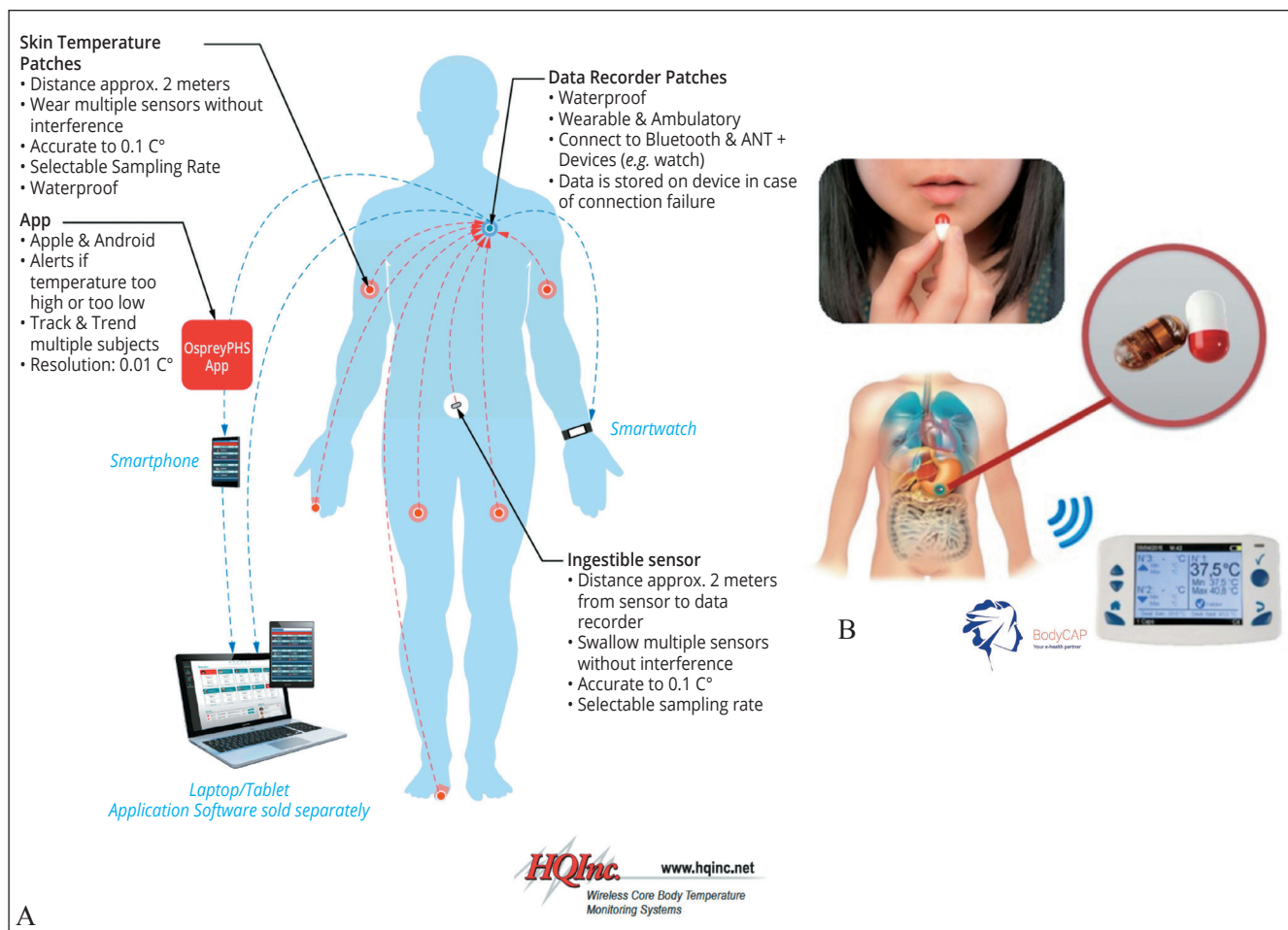
Figure 5.—Core temperature monitoring by HQInc (A) and BodyCap (B).
