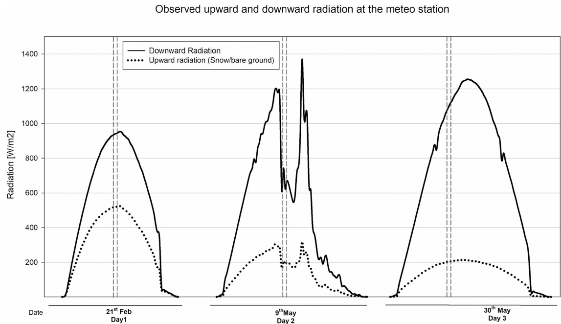
Fig. 5. Upward and downward radiation observed at the automatic weather stations of Izas Experimental Catchment for the three acquisition dates. Vertical dashed lines denote the time interval of UAV acquisitions.
