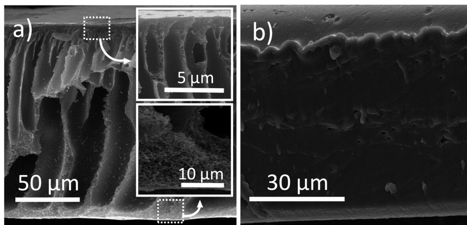
Fig. 1. Cross-section images of the PFS support (a) and the Pebax® 3533 dense membrane prepared by the conventional casting-solution method (b). Insets correspond to the top and bottom sides of the PSF support.
