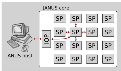
Fig. 1. Conceptual architecture of a Janus system, including the cluster of Simulation Processors (SPs), the Input-Output Processor (IOP) and the host PC.
