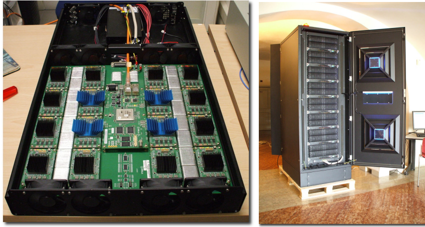
Fig. 2. Left: a Janus processing-board with 16 SPs; Right: a large Janus system with 16 processing-boards, 256 SPs and 8 host PCs.
