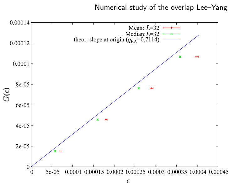
Figure 11. Integrated density of the zeros, for the largest lattice L = 32 and lowest temperature \beta = 1.4 using the average of zeros. We have also plotted the median values. We have marked the expected slope at the origin, using the Edwards–Anderson order parameter computed in [20] for the L = 32 lattice.
