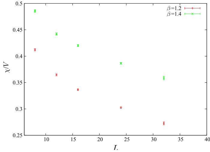
Figure 4. \chi/V = \overline{\langle q^2 \rangle} versus the lattice size for \beta = 1.2 and 1.4 . Notice that none of the temperatures have reached the plateau asymptotic value.
