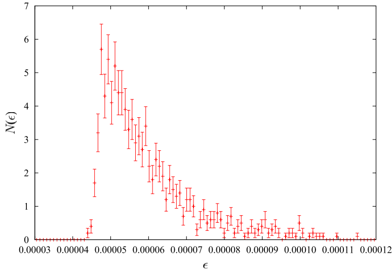
Figure 9. Histogram ( N(\epsilon) versus \epsilon ) for the first 1000 zeros computed for L = 32 and \beta = 1.4 . Notice the lack of symmetry of the histogram and the presence of events for large values of the zeros.
