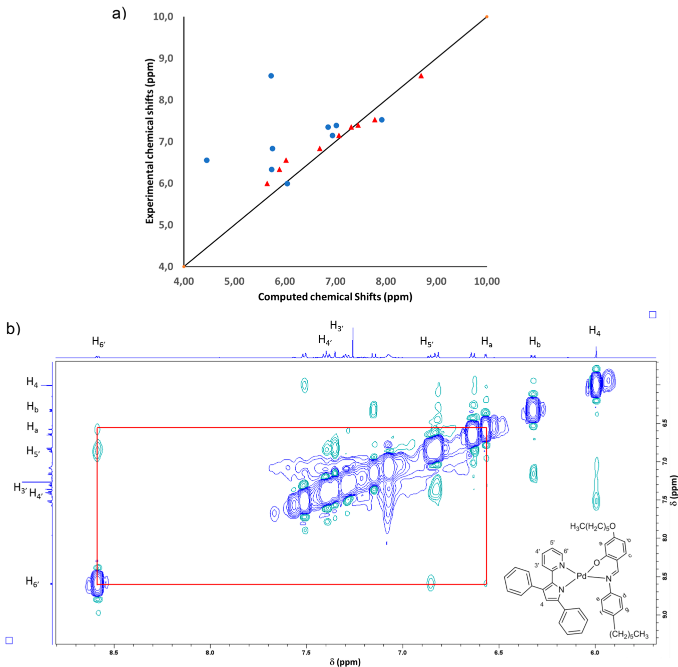
Figure 3. (a) Correlation between computed and experimental ^1\text{H} NMR chemical shifts. Red triangle 2 trans_{(N_{pyr}\cdots O)} and blue circles 2 cis_{(N_{pyr}\cdots O)} . (b) 2D-NOESY ^1\text{H} NMR for 2 ; the red line shows the correlation between H_{6'} and H_a .
