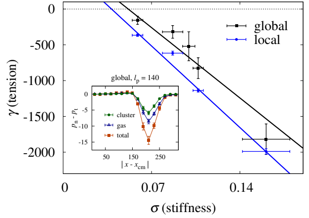
Fig. 3 The main figure correlates the interfacial tension and the stiffness, showing that the tension becomes more negative with increasing stiffness. This suggests that the same dynamics that produces a positive stiffness yields a negative interfacial tension. The black points correspond to measurements in the global frame (described in Sec. 3), while the blue points correspond to measurements in the local frame of the interface (described in Sec. 4). The inset shows the difference between normal and tangential pressure that determines the integrand in Eq. 11, broken down into cluster and gas contributions, highlighting the significant net-negative contributions from both cluster and gas particles.
