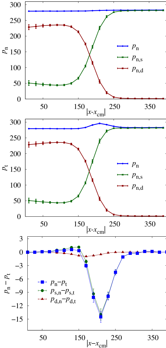
Fig. 9 Normal (top) and tangential (middle) pressure broken down into swim, interaction and total parts. The bottom panel shows the various contributions (total, swim and interaction) to the difference p_n - p_t as a function of the distance x from the dense phase center of mass, for \ell_p = 140 . This difference is the integrand in the expression for the tension, Eq. (11).
