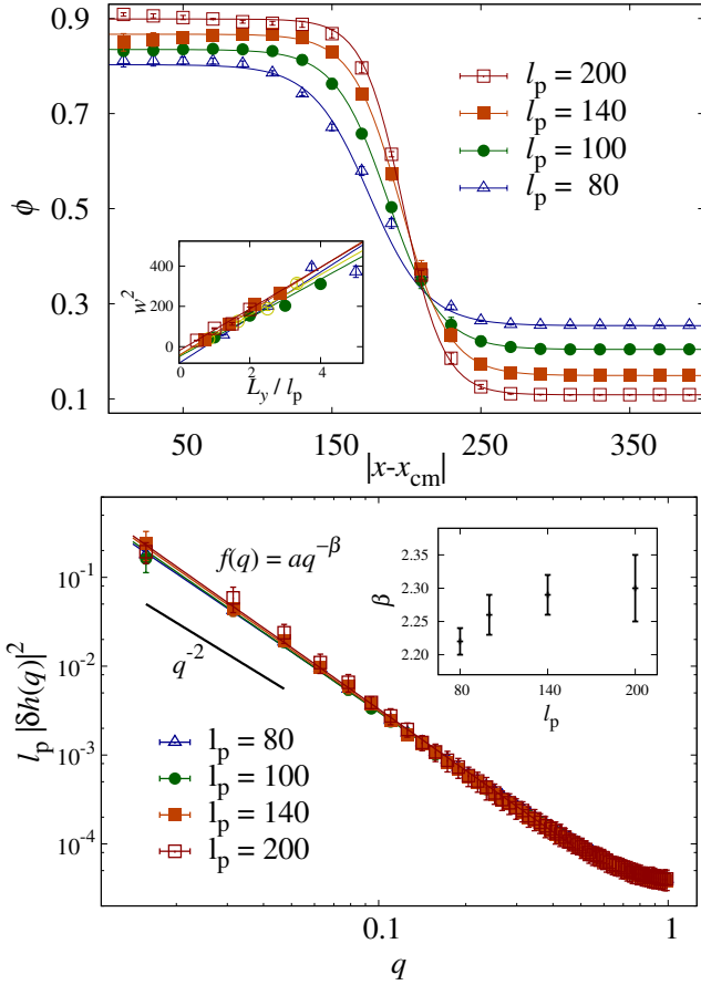
Fig. 2 Top: density profiles in the interface frame, for varying persistence. [Inset] Scaling of w^2 as a function of L_y/\ell_p , for comparison to Eq. 7. Bottom: Interface height fluctuation spectrum for systems with L_y = 400 , collapse for several values of \ell_p . The equilibrium expectation \langle |\delta h(q)|^2 \rangle \sim q^{-2} is shown as a solid black line. The collapse of \ell_p |\delta h(q)|^2 , signifies the clear dependence of interfacial fluctuations on persistence. [Inset] Best fit exponent characterizing the initial decay of the interface modes as a function of \ell_p .
