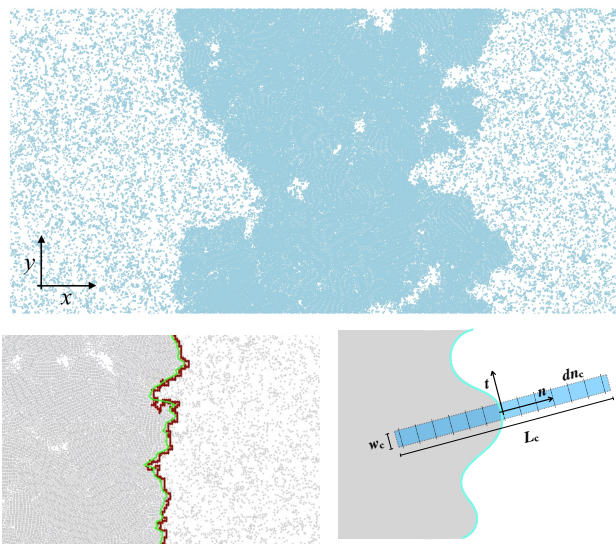
Fig. 1 Top: A snapshot of a system composed of roughly 2 \times 10^5 active Brownian particles of radius r_0 undergoing spontaneous separation into dense and dilute phases. The persistence length of the particles (defined in the text) is \ell_p = 100r_0 ; the area fraction is \phi = 0.5 and phase separation into a strip geometry is attained by choosing the aspect ratio of the simulation box to be L_x/L_y = 2 , with periodic boundary conditions (here L_x = 1600r_0 ). Bottom left: A demonstration of two methods for identifying the interface. The red curve results from a contour-finding algorithm that captures all overhangs and allows for local curvature measurements, while the green curve considers only the outermost particles at each value of y and can be used to obtain the spectrum of the interface height fluctuations (see Appendix A for details). Bottom right: A schematic of the the local frame we use to measure dynamical quantities near the interface (see Appendix B for details).
