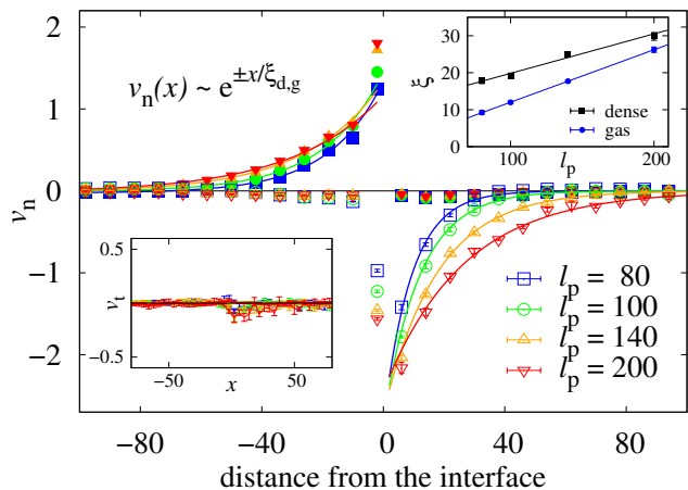
Fig. 8 The main figure shows the normal velocity v_n of particles measured in the local frame and averaged along the interface. The solid (open) symbols correspond to particles in the dense (gas) phase. The positive, outward-moving average velocity just inside the dense phase is balanced by the negative inward-moving average velocity just inside the gas phase. Within each phase, the normal average velocity is finite within a surface layer of thickness \xi_d (dense) and \xi_g (gas) and decays exponentially. The solid lines are fits to the exponential decay. The top right inset shows \xi_{d,g} extracted from those fits as functions of \ell_p . The solid lines are fits that show the linear growth of \xi_{d,g} with persistence. The bottom left inset shows that the signed tangential component of velocity is zero at the interface because particles travel without preference in either direction tangent to the interface.
