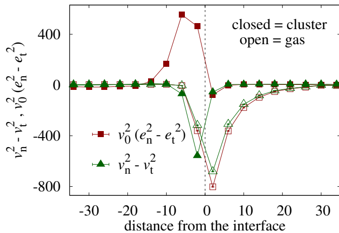
Fig. 4 We use the local frame along the phase boundary to illuminate the complex dynamics near the interface—in particular the anisotropy of director and velocity. The x -axis shows the distance from the interface measured along the normal, as shown in Fig. 1. Near the interface, the average director field shows an excess of inward pointing swim force just inside the cluster and an excess of transverse swim force just inside the gas. The anisotropy of the resulting motion shows that the gas moves with its director field, but the cluster self-shears as its surface particles move tangentially.
