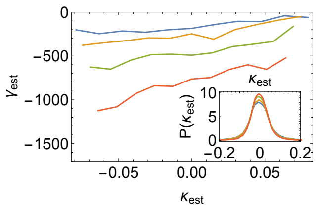
Fig. 5 Correlation between the estimated local surface tension and local curvature for \ell_p = 80, 100, 140, 200 (top to bottom). Negative and positive curvature values correspond to mountains and valleys of the interface, respectively. The correlation between curvature and tension provides a Marangoni-like effect which allows the interface to stabilize itself. [Inset] Probability distribution of local curvatures for the same parameters (where higher values of \ell_p have a more peaked distribution of curvature).
