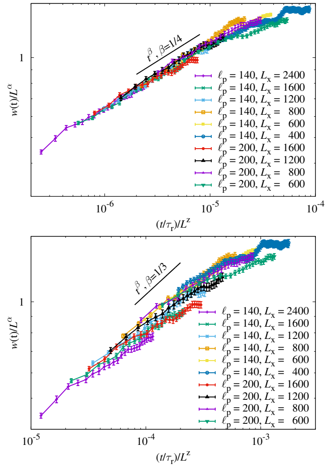
Fig. 6 The growth of the interfacial width w(t) starting from a flat configuration for several \ell_p and system sizes is shown. We present a scaling collapse according to the Edwards-Wilkinson (top) and Kardar-Parisi-Zhang (bottom) critical exponents. Here \alpha = 1/2 , z = \alpha/\beta , \beta_{\text{KPZ}} = 1/3 , \beta_{\text{EW}} = 1/4 .
