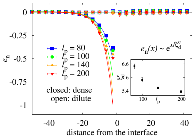
Fig. 7 The main figure shows the normal component of the polarization e_n measured in the local frame and averaged along the interface. This is proportional to the average local swim force per particle. The solid (open) symbols correspond to particles in the dense (gas) phase. The data show that there is an excess of inwardly polarized particles in a surface layer of thickness \xi_d^e in the dense phase, but not in the gas. The length \xi_d^e has been extracted with an exponential fit to the decay of e_n and is shown in the inset as a function of \ell_p . It is found to decay with increasing persistence. The net tangential component of polarization (not shown) remains zero at the interface because particles travel without preference in either direction tangent to the interface.
