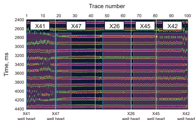
Fig. 16. Third comparison of time-lapse imaging results of background noise data (July 20–August 20).
