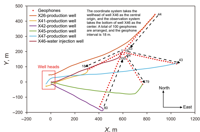
Fig. 11. Observation system resembling a star layout (The black numbers and black dotted lines are the geophones numbers and layout directions.)
