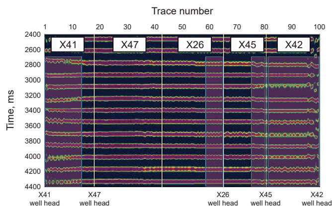
Fig. 14. First comparison of time-lapse imaging results of background noise data (July 20–July 31, the white vertical line is the dividing line between the data of the five wells).
