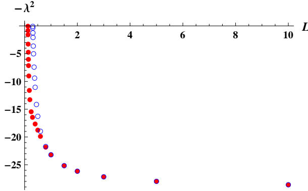
Figure 4.6: Negative energy of symmetric (red dots) and antisymmetric (blue dots) bound states locate in the domain between the q - \bar{q} pair for \alpha = 0.4 and \Lambda = 5
