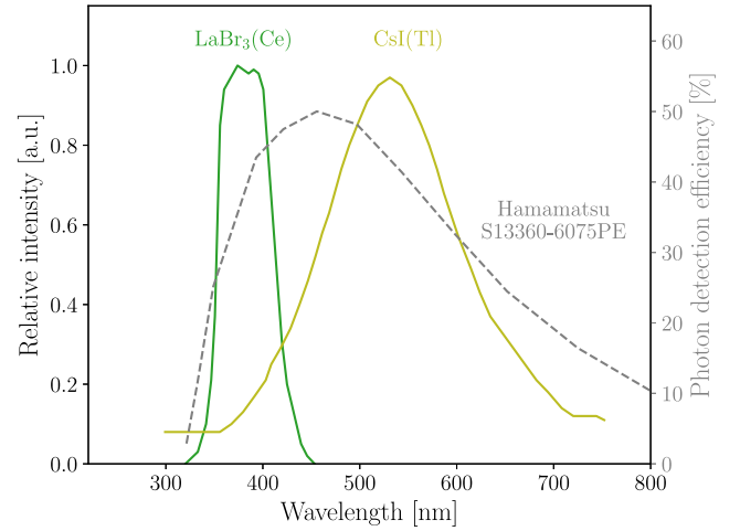
Fig. 5. Emission spectrum of the scintillating crystals \text{LaBr}_3(\text{Ce}) (in green) and \text{CsI}(\text{Tl}) (in yellow) compared with Hamamatsu MPPC S13360-6075PE PDE (in gray, right axis). Source: Data taken from vendors [33,40,41].
