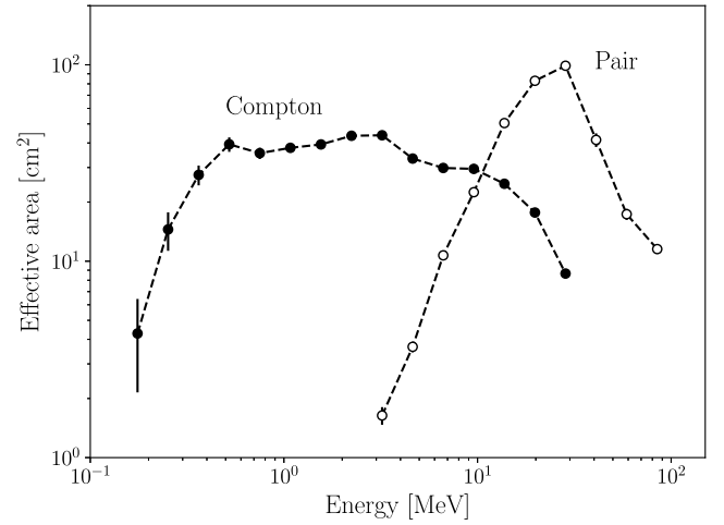
Fig. 13. Effective area of the COCOA telescope for Compton (black dots) and pair-production (white dots) events as a function of the gamma ray energy. The value used for the sensitivity calculation corresponds to the sum of the two components.
