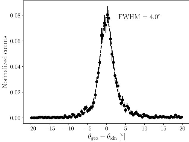
Fig. 10. ARM for on-axis 1 MeV gamma rays producing two-site events in the COCOA detector, obtained with a Geant4 simulation. The dashed line corresponds to a double Gaussian fit with FWHM = 4.0°.
