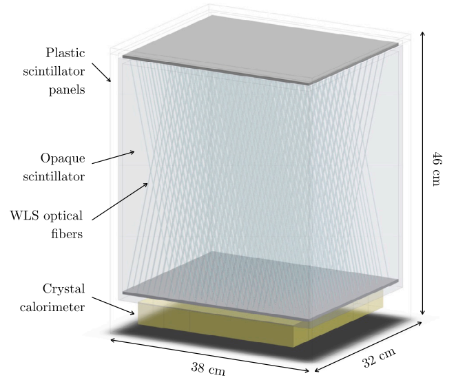
Fig. 2. CAD drawing of the COCOA detector. It comprises an opaque scintillator intersected by a grid of wavelength-shifting fibers, with a crystal calorimeter placed on the bottom. It is surrounded by plastic scintillator panels to reject the charged particles background.
