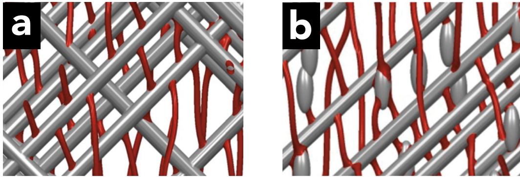
Fig. 23. Optimization of pinning performance for vortices (red) misaligned with a pinning landscape that consists of columnar defects (gray cylinders): Panel (a) shows a simulation snapshot of played columnar defects and (b) a mixed pinning landscape including columnar defects and elongated nanoparticles (gray ellipses). These simulation snapshots are reprinted with permission from [32] (Copyright Wiley-VCH GmbH).
