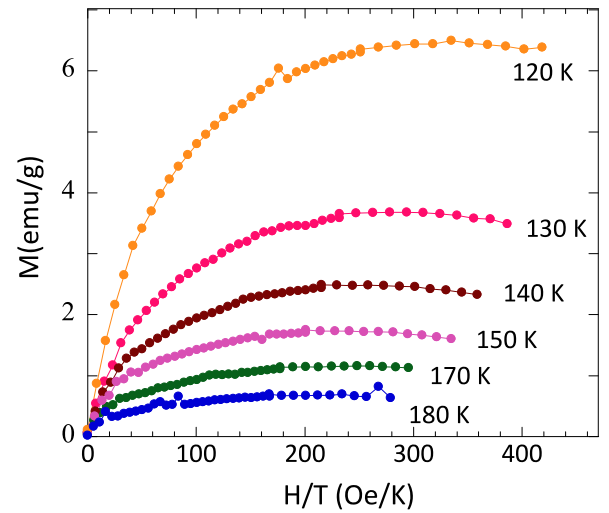
Fig. 4. (Colour online) Magnetization M versus H/T plots for representative temperatures in the GP regime T_C < T < T_G . The lines are intended as guides for the eye.
