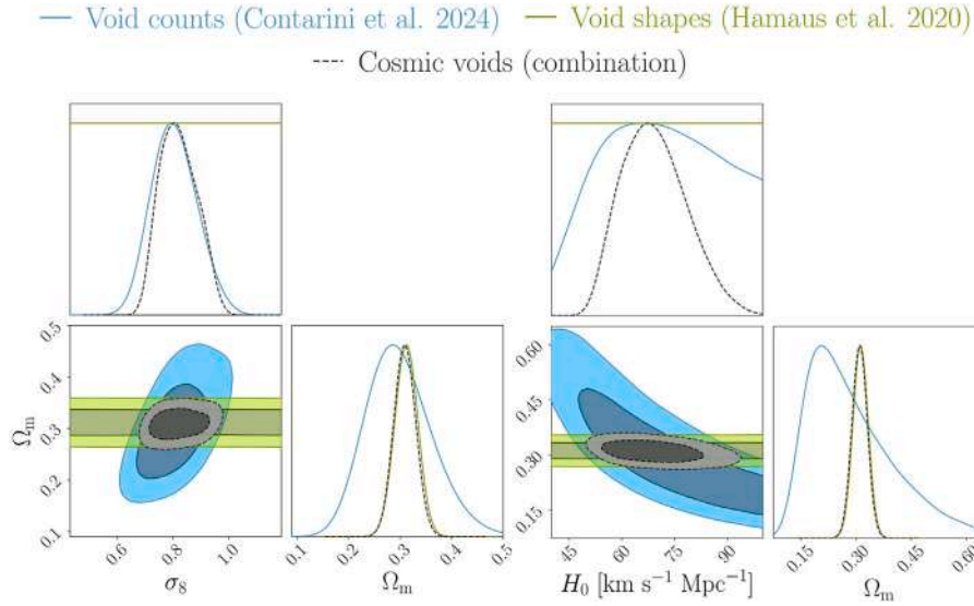
Fig. 46. Confidence contours from void counts (light blue, [1798]) and void shape distortions (green, [1799]) of the BOSS DR12 voids, and their combination (black) as independent constraints on \Omega_m , H_0 and \sigma_8 . Adapted from [1798], licensed under Creative Commons Attribution 4.0 International (CC BY 4.0). (For interpretation of the references to colour in this figure legend, the reader is referred to the web version of this article.)
