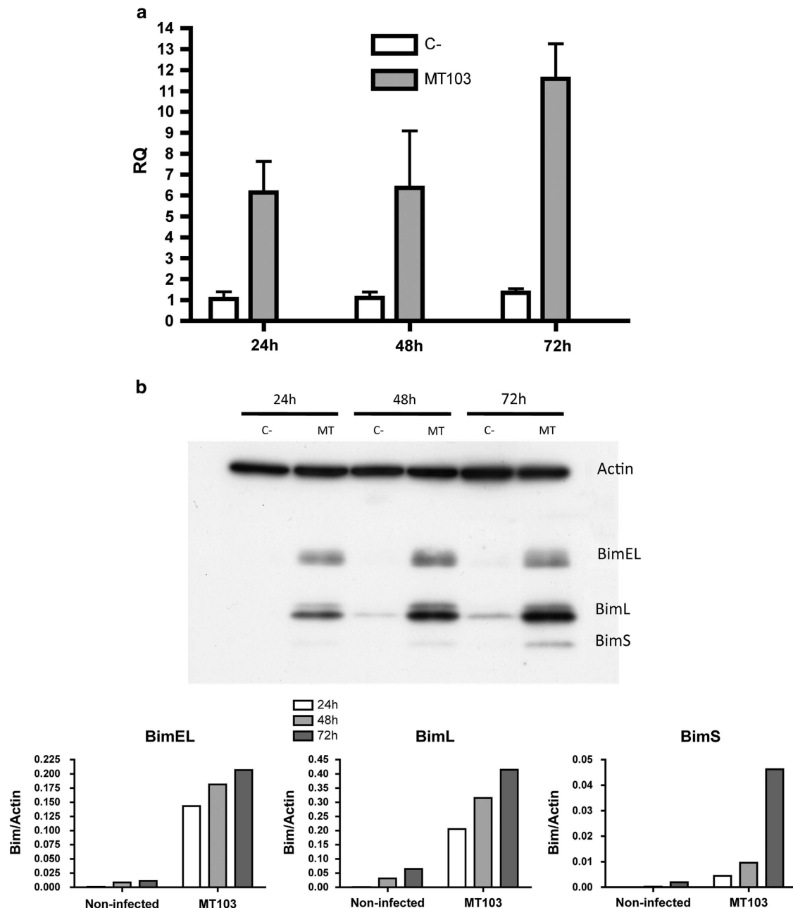
Figure 2 MT103 upregulates Bim in J774 cells. J774 cells were infected with MT103 (MOI 10:1) up to 72 h. Bim expression was analysed by RT-qPCR (a), or by western blot (b) at 24 h, 48 h and 72 h post infection. (a) Data in the graph are represented as mean \pm S.E.M. of three independent experiments. (b) Quantification of the western blot is represented as the ratio of Bim/Actin densities. A representative blot of three independent is shown in the figure
