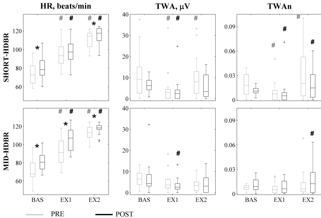
Figure 5: HR and TWA amplitude distribution at each AP test step (BAS, EX1, EX2), computed before (grey) and after (black) five days (top panels) and after twenty-one days (bottom panels) of HDBR. *: p < 0.05 , PRE vs POST. #: p < 0.05 , vs previous step.
