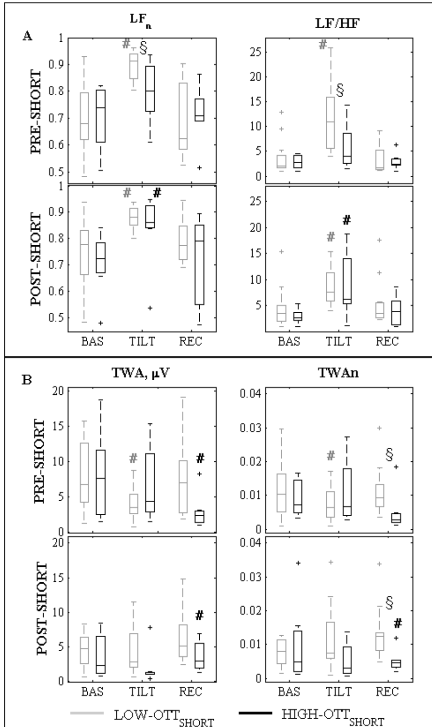
Figure 4: HRV (A) and TWA (B) indices computed for LOW-OTT SHORT (grey) and HIGH-OTT SHORT (black) groups, before and after the SHORT-HDBR (up and bottom panels, respectively). #: p < 0.05 , vs BAS. §: p < 0.05 , LOW-OTT SHORT vs HIGH-OTT SHORT .
