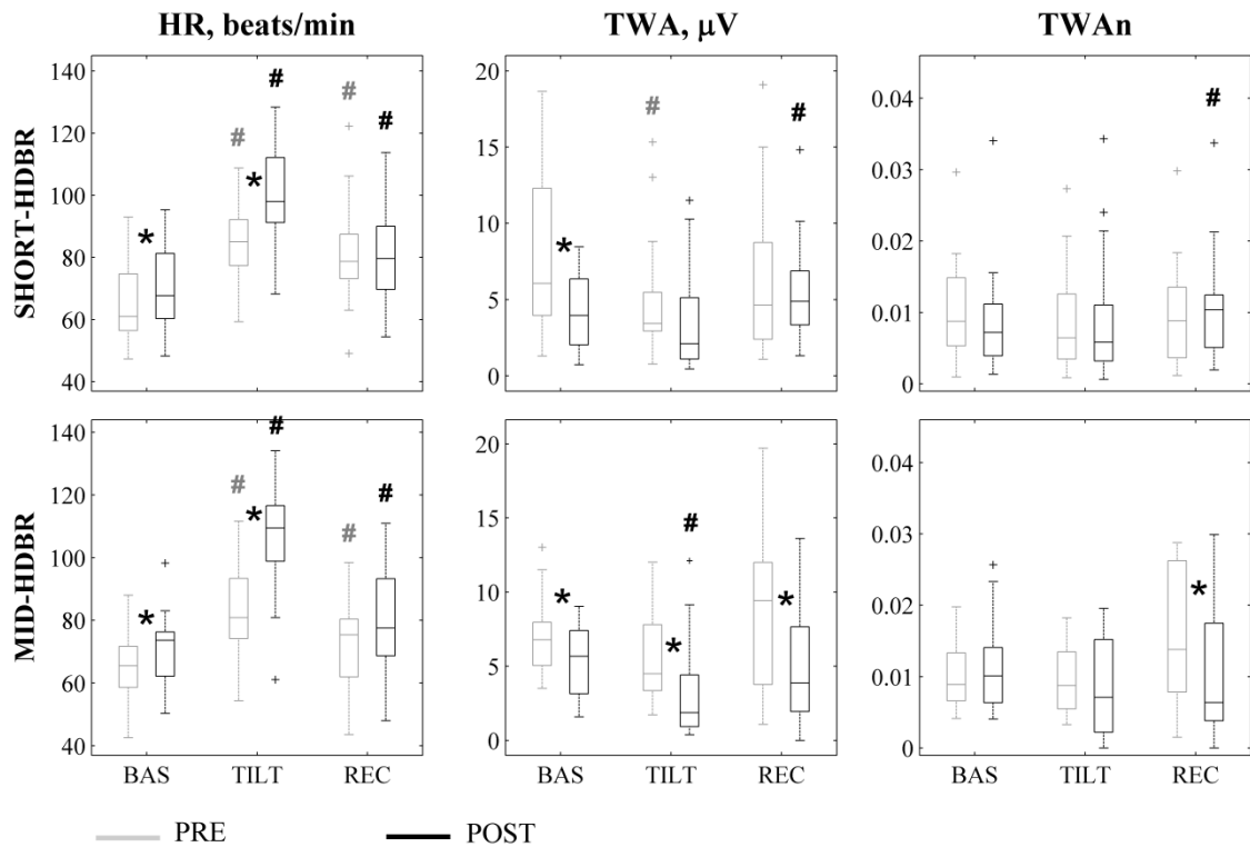
Figure 3: Cumulative results for HR and TWA amplitudes, reported as absolute and normalized (TWAn), obtained in SHORT (top) and in MID (bottom) campaigns during orthostatic tilt test (*: p < .05 , PRE vs POST, #: p < .05 vs BAS).
