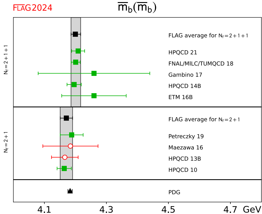
FIG. 7. The b -quark mass for N_f = 2+1 and 2+1+1 flavors. The updated PDG value from Ref. [274] is reported for comparison.
