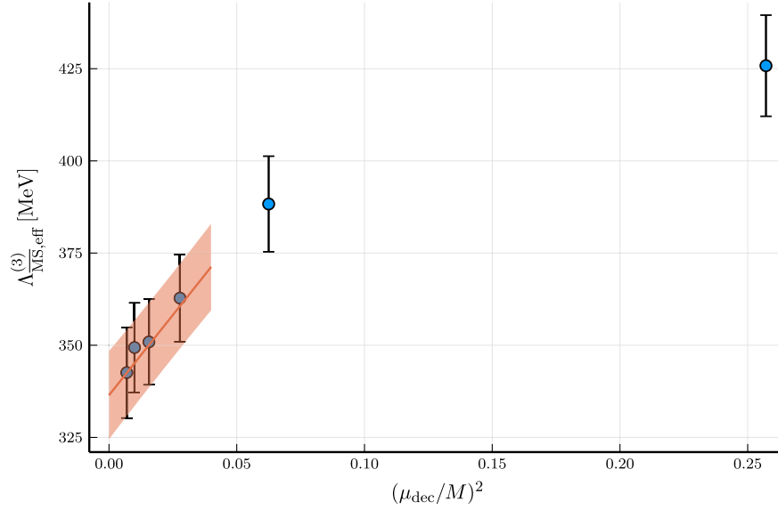
FIG. 37. The decoupling limit M \rightarrow \infty in ALPHA 22, Ref. [80].
