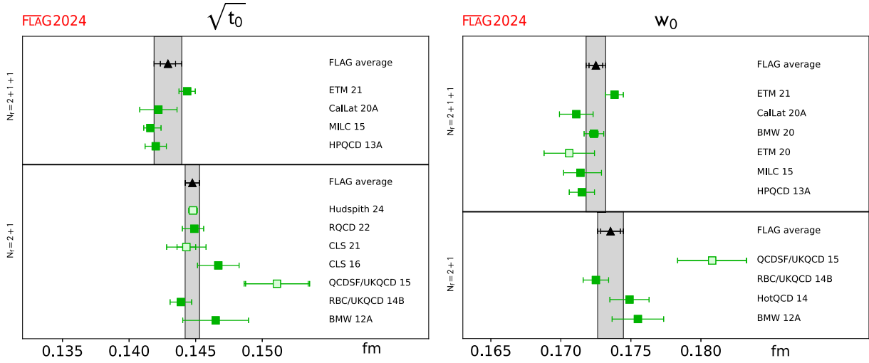
FIG. 51. Results for gradient flow scales.
