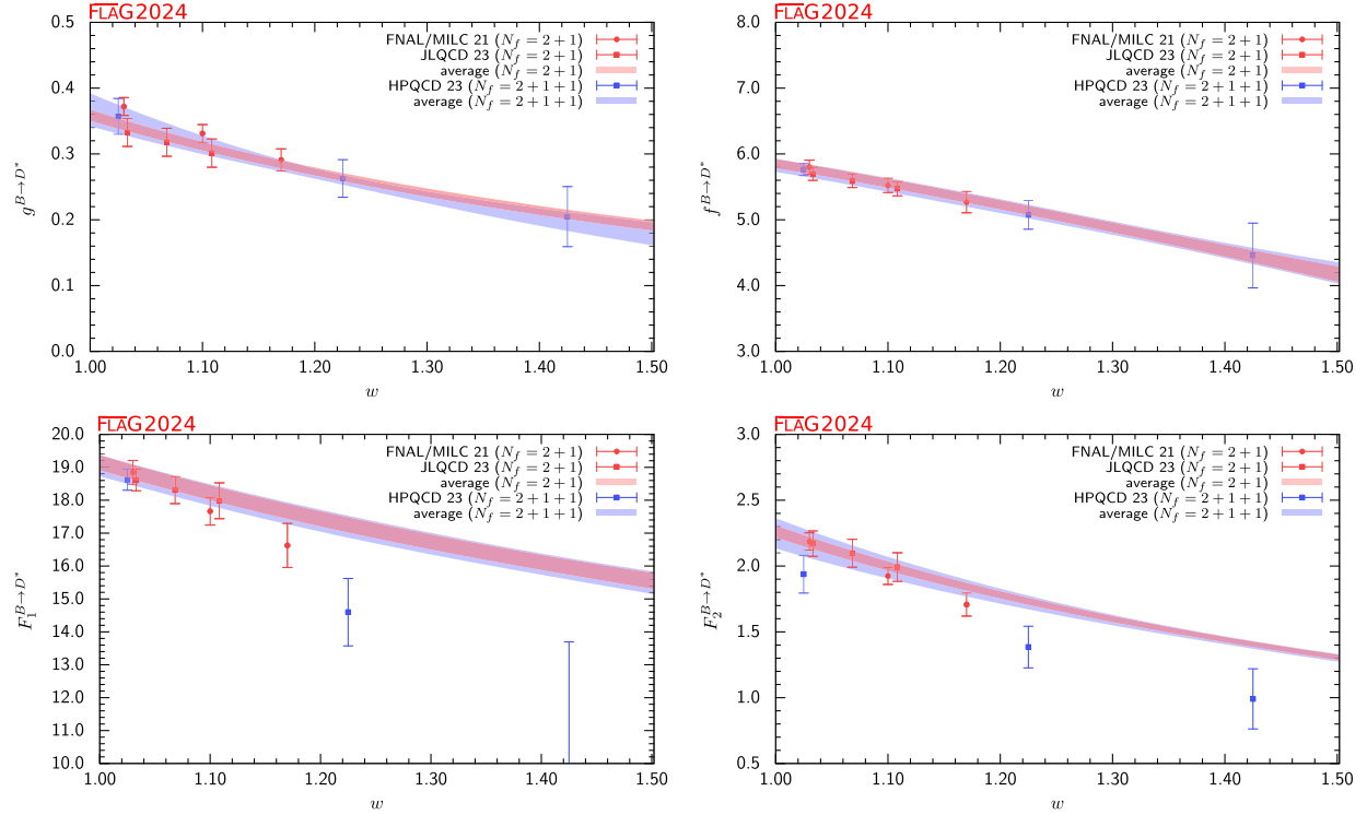
FIG. 33. The form factors g(q^2) , f(q^2) , F_1(q^2) , and F_2(q^2) for B \rightarrow D^* \ell \nu plotted as a function of w . The red (blue) band displays our preferred (N_g, N_f, N_{F_1}, N_{F_2}) = (2, 3, 3, 2) BGL fit (eight parameters) to experimental and N_f = 2 + 1(2 + 1 + 1) lattice data. The constraints at zero and maximum recoil are imposed exactly. No use of unitarity constraints and priors has been made.
