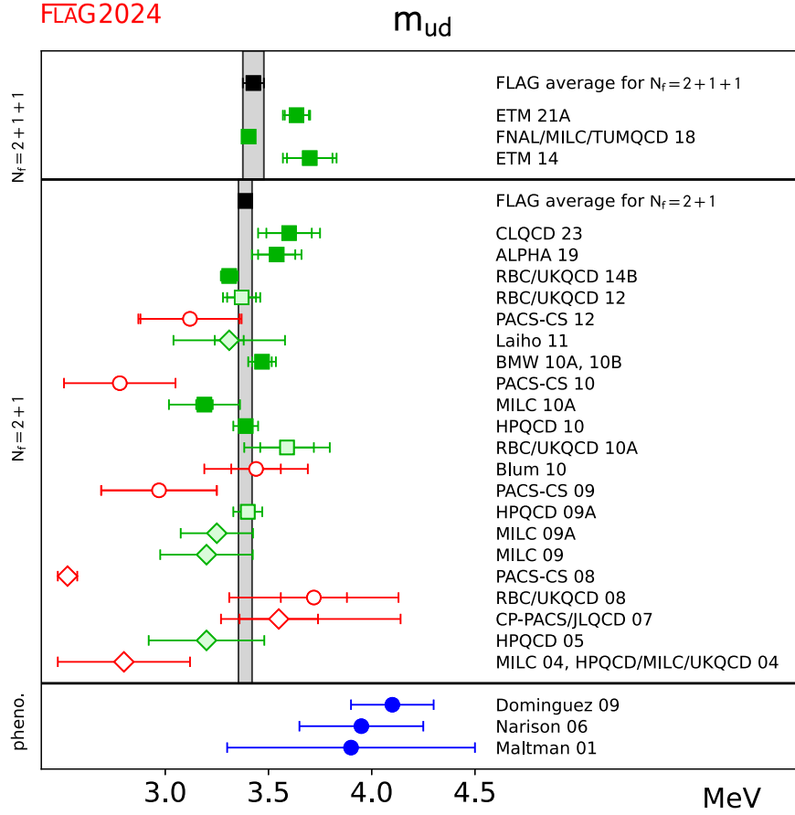
FIG. 2. Mean mass of the two lightest quarks, m_{ud} = \frac{1}{2}(m_u + m_d) . The bottom panel shows results based on sum rules [247,250,252] (for more details see Fig. 1).
