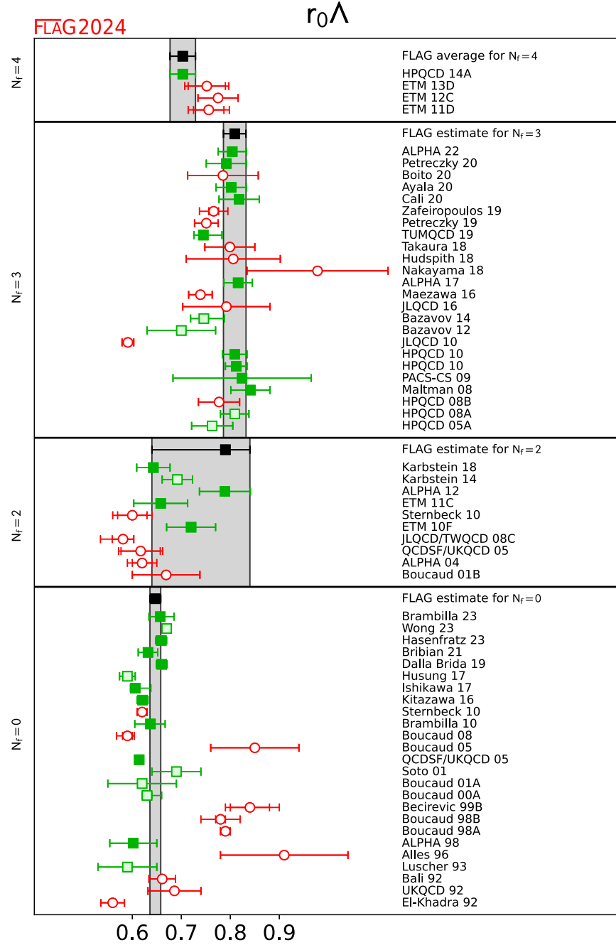
FIG. 38. r_0 \Lambda_{\overline{\text{MS}}} estimates for N_f = 0, 2, 3, 4 flavors. Full green squares are used in our final ranges, pale green squares also indicate that there are no red squares in the color coding but the computations were superseded by later more complete ones or not published, while red open circles mean that there is at least one red square in the color coding.
