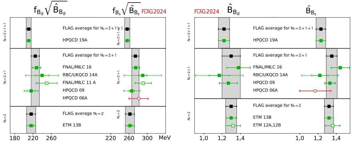
FIG. 23. Neutral B - and B_s -meson-mixing matrix elements and bag parameters [values in Table 35 and Eqs. (182), (185), (188), (183), (186), (189)].
