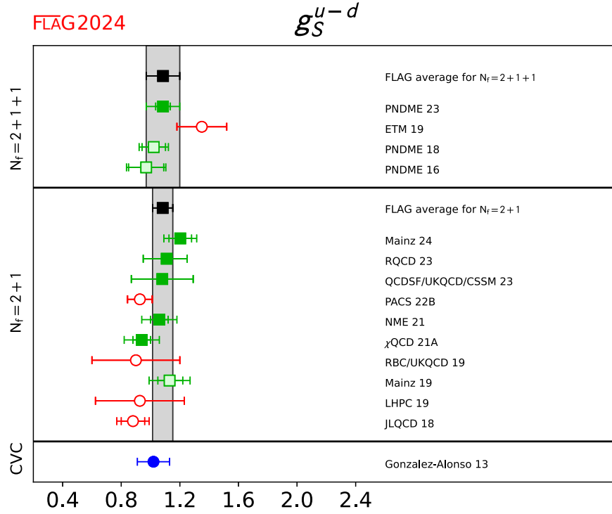
FIG. 43. Lattice results and FLAG averages for the isovector scalar charge g_S^{u-d} for N_f = 2+1 and 2+1+1 flavor calculations. Also shown is a phenomenological result obtained using the conserved vector current (CVC) relation [982] (circle).
