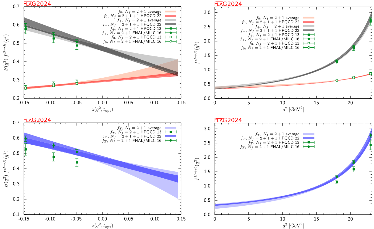
FIG. 27. The B \rightarrow K form factors f_+(q^2) , f_0(q^2) and f_T(q^2) plotted versus z (left panels) and q^2 (right panels). In the plots as a function of z , we remove the Blaschke factors. See text for a discussion of the datasets. The light-shaded gray, salmon and blue bands display our preferred N^+ = N^0 = N^T = 3 BCL fit (eight parameters) to the N_f = 2 + 1 lattice results. The dark-shaded gray, salmon and blue bands display the N_f = 2 + 1 + 1 HPQCD 22 results [492].
