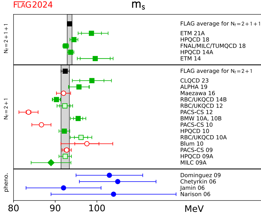
FIG. 1. \overline{MS} mass of the strange quark (at 2 GeV scale) in MeV. The upper two panels show the lattice results listed in Tables 7 and 8, while the bottom panel collects sum rule results [247–251]. The diamond represents a result based on perturbative renormalization. The squares and open circles denote results based on nonperturbative renormalization. The black squares and the gray bands represent our averages (32) and (34). The significance of the colors is explained in Sec. II.
