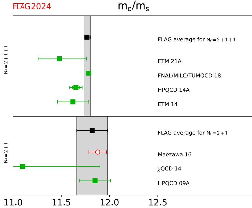
FIG. 6. Lattice results for the ratio m_c/m_s listed in Table 14 and the FLAG averages corresponding to 2+1 and 2+1+1 quark flavors. The latter average includes a stretching factor of 1.4 on the error due to a poor \chi^2 from our fit.
