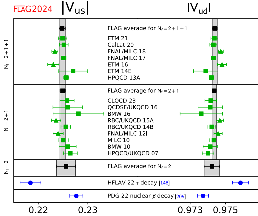
FIG. 12. Results for |V_{us}| and |V_{ud}| that follow from the lattice data for f_+(0) (triangles) and f_{K^\pm}/f_{\pi^\pm} (squares), on the basis of the assumption that the CKM matrix is unitary. The black square and the gray band represent the average for each value of N_f . For comparison, the figure also indicates the results obtained if the data on nuclear \beta decay and inclusive hadronic \tau decay is analyzed within the Standard Model.
