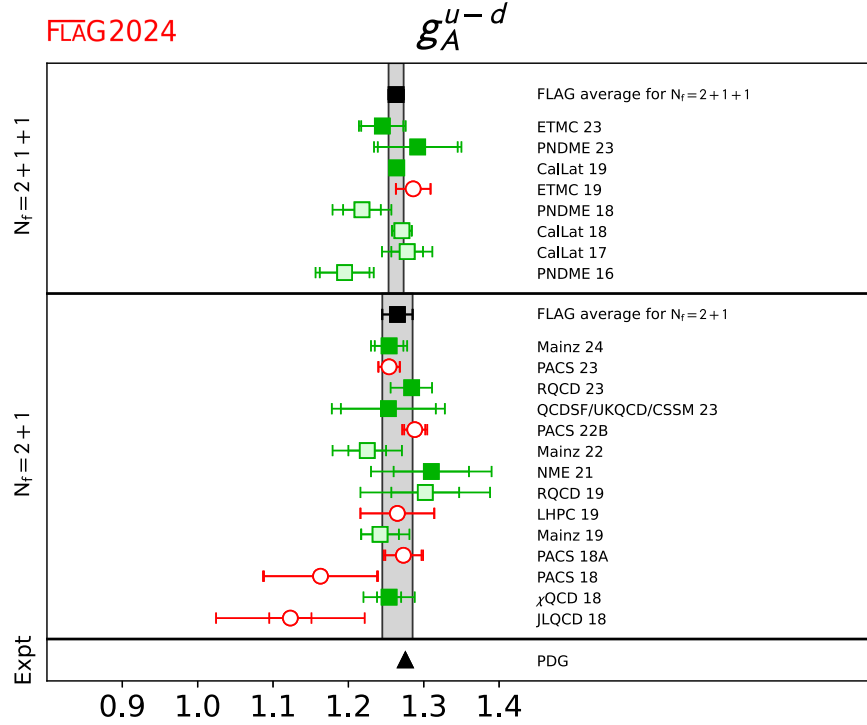
FIG. 42. Lattice results and FLAG averages for the isovector axial charge g_A^{u-d} for 2+1 and 2+1+1 flavor calculations. Also shown is the experimental result as quoted in the PDG [205].
