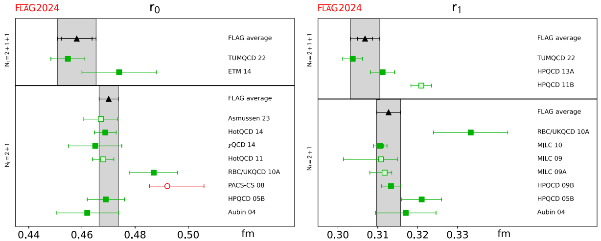
FIG. 52. Results for potential scales.
