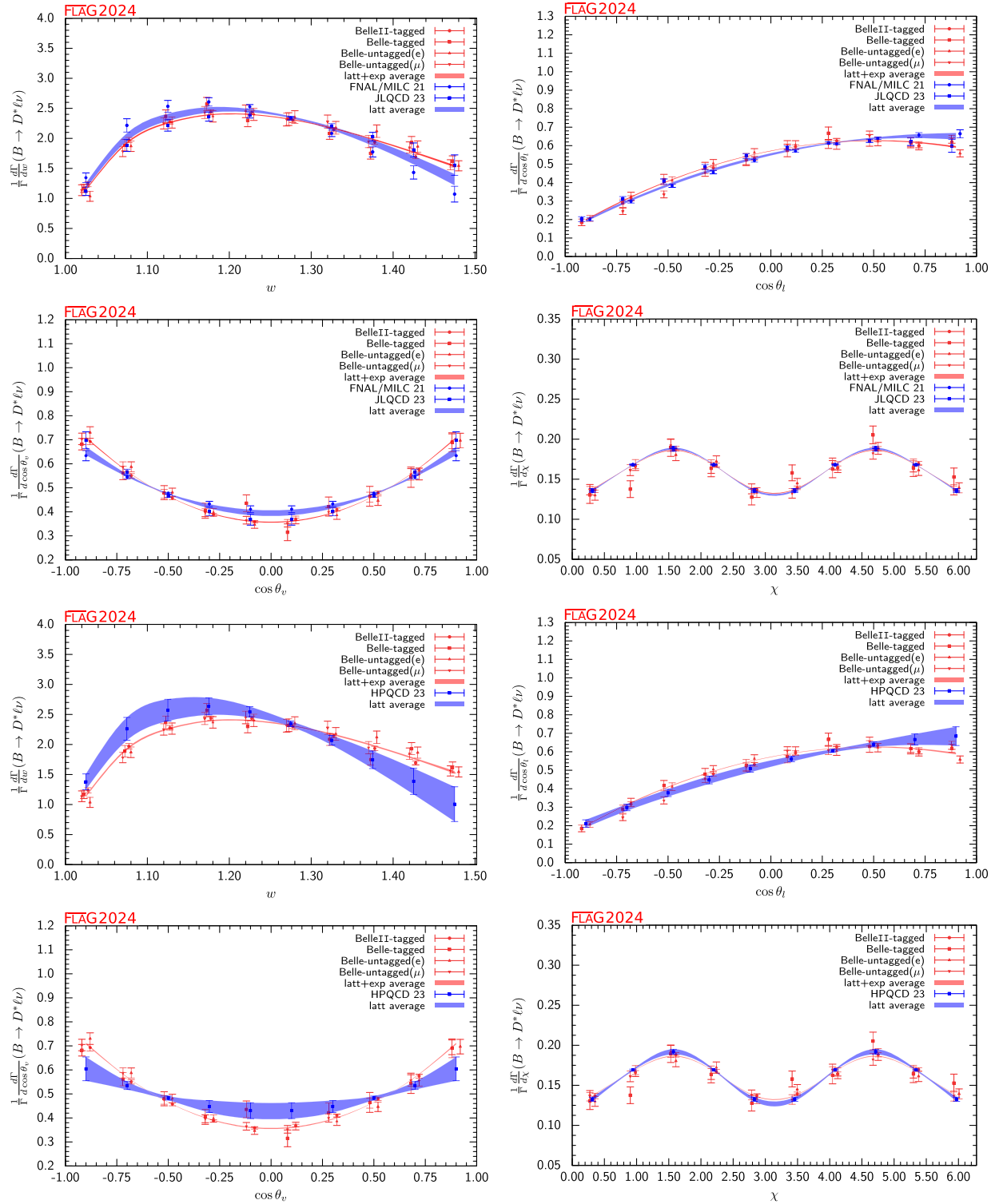
FIG. 34. Normalized differential decay rates with respect to the variables w , \cos \theta_l , \cos \theta_v and \chi . The red (blue) band displays our preferred (N_g, N_f, N_{F_1}, N_{F_2}) = (2, 3, 3, 2) BGL fit (eight parameters) obtained from lattice calculations with (without) the inclusion of experimental data. The constraints at zero and maximum recoil are imposed exactly. No use of unitarity constraints and priors has been made. The top and bottom four distributions are obtained using N_f = 2 + 1 and N_f = 2 + 1 + 1 lattice calculations, respectively.
