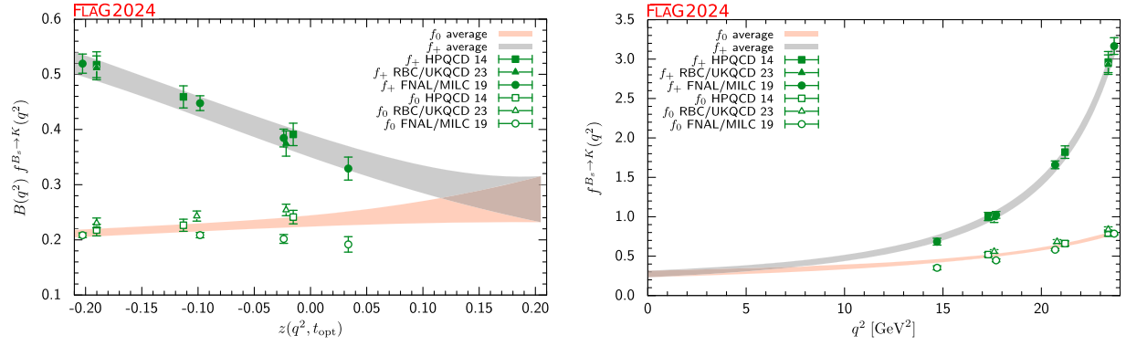
FIG. 26. The form factors f_+(q^2) and f_0(q^2) for B_s \rightarrow K \ell \nu plotted versus z (left panel) and q^2 (right panel). In the left plot, we remove the Blaschke factors. See text for a discussion of the datasets. The gray and salmon bands display our preferred N^+ = N^0 = 4 BCL fit (seven parameters).
