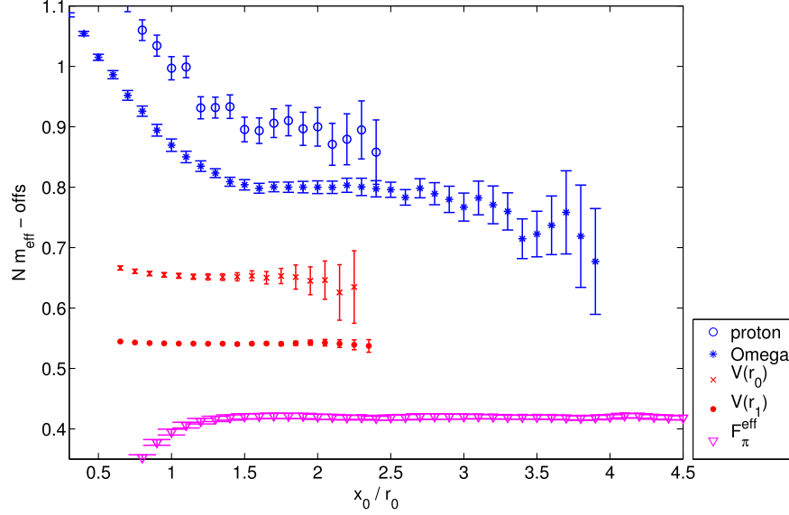
FIG. 50. Effective masses for M_{\text{proton}} [1062], M_{\Omega} [1063], V(\approx r_0) , V(\approx r_1) [717] and f_{\pi} [1064] on N_f = 2 CLS ensemble N6 with a = 0.045 fm, M_{\pi} = 340 MeV on a 48^3 \times 96 lattice [1064]. All effective “masses” have been scaled such that the errors in the graph reflect directly the errors of the determined scales. They are shifted vertically by arbitrary amounts. Figure from Ref. [824]. Note that this example is at still favorably large quark masses. The situation for M_{\text{proton}} becomes worse closer to the physical point, but may be changed by algorithmic improvements.
