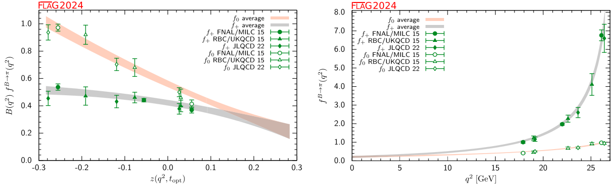
FIG. 25. The form factors f_+(q^2) and f_0(q^2) for B \rightarrow \pi \ell \nu plotted versus z (left panel) and q^2 (right panel). In the left plot, we removed the Blaschke factors. See text for a discussion of the dataset. The gray and salmon bands display our preferred N^+ = N^0 = 3 BCL fit (five parameters).
