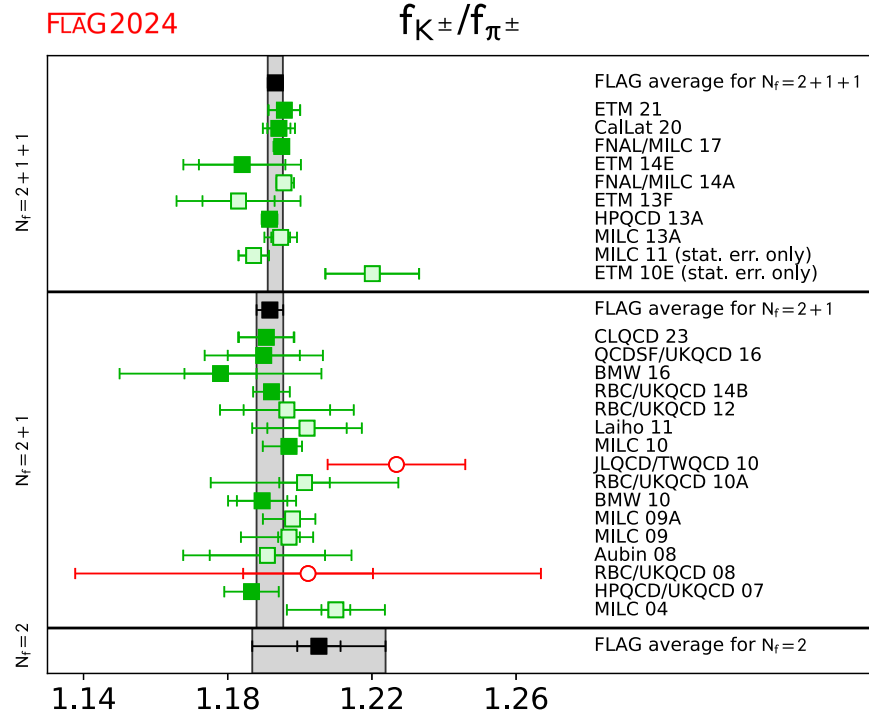
FIG. 9. Comparison of lattice results for f_{K^\pm}/f_{\pi^\pm} . This ratio is obtained in pure QCD including the isospin-breaking correction (see Sec. V C). The black squares and gray bands indicate our averages in Eqs. (76) and (77).
