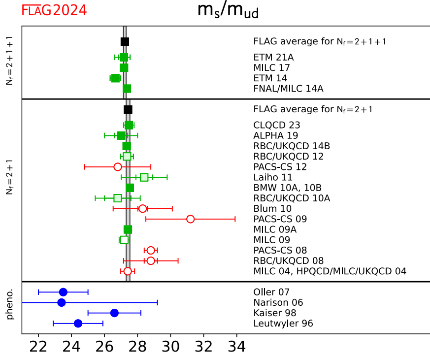
FIG. 3. Results for the ratio m_s/m_{ud} . The upper part shows the lattice results listed in Table 9 together with the FLAG averages for each value of N_f . The lower part shows results obtained from \chi PT and sum rules [250,253–256].
