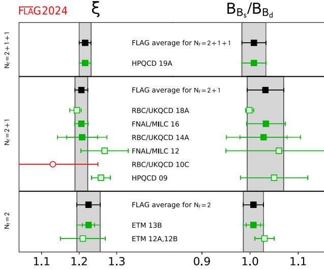
FIG. 24. The SU(3)-breaking quantities \xi and B_{B_s}/B_{B_d} [values in Table 36 and Eqs. (184), (187), (190)].
