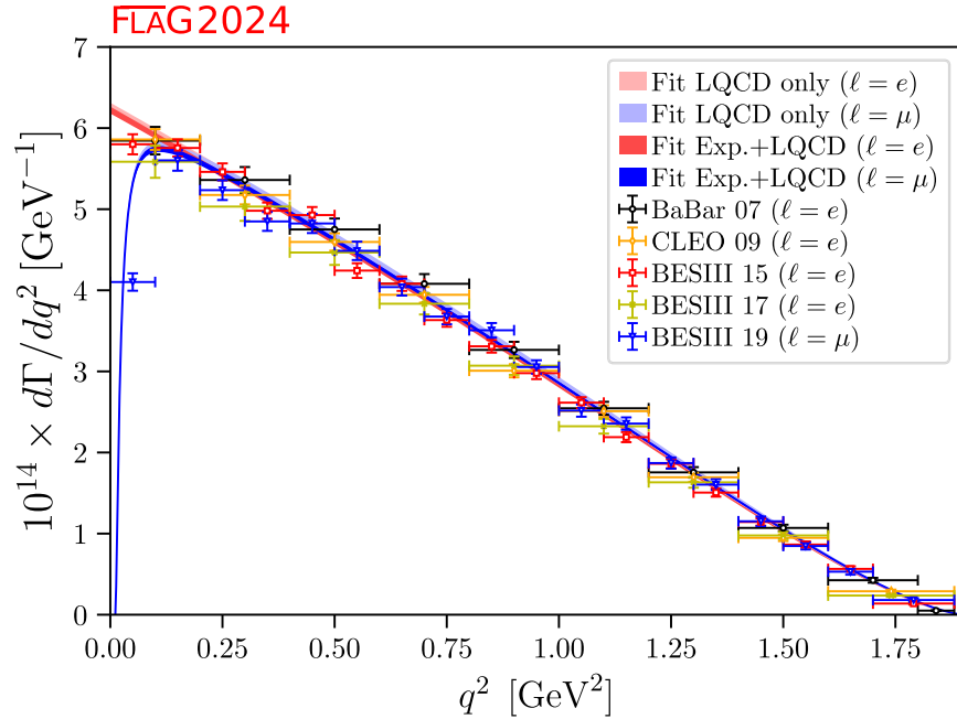
FIG. 19. Our fits to the D \rightarrow K\ell\nu differential decay rates used to determine |V_{cs}| , with experimental inputs from Refs. [472, 505–508] and lattice inputs from ETM17D [63], HPQCD 21A [65], and FNAL/MILC 22 [123].
