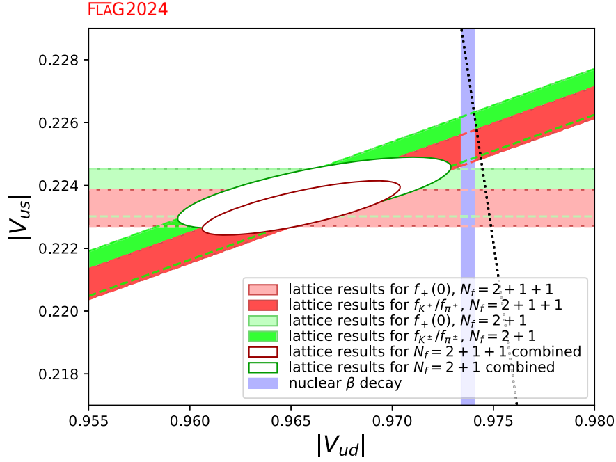
FIG. 10. The plot compares the information for |V_{ud}| , |V_{us}| obtained using lattice QCD for N_f = 2 + 1 and N_f = 2 + 1 + 1 with |V_{ud}| extracted from nuclear \beta transitions Eq. (69). The black dotted line indicates the correlation between |V_{ud}| and |V_{us}| that follows if the CKM-matrix is unitary.
