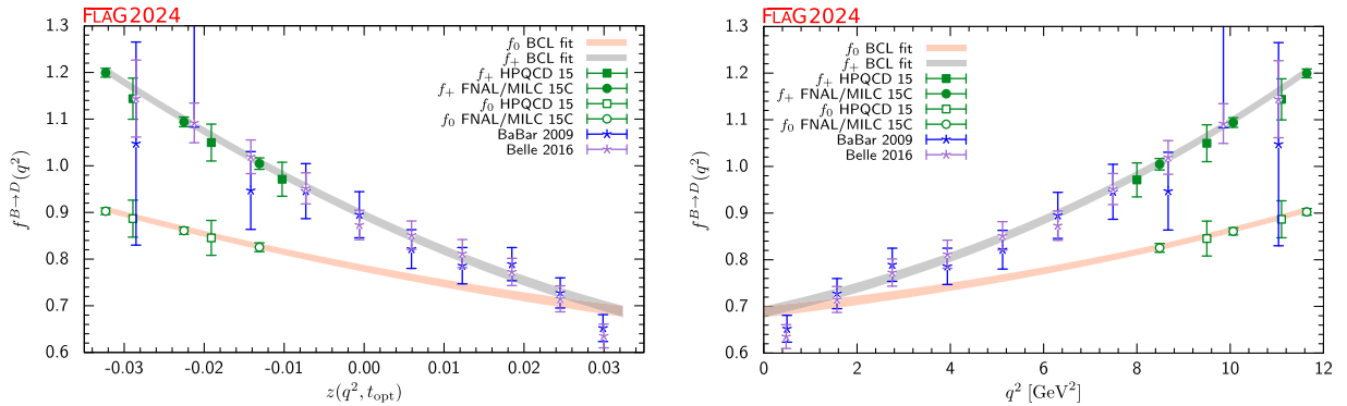
FIG. 32. Lattice and experimental data for f_+^{B \rightarrow D}(q^2) and f_0^{B \rightarrow D}(q^2) versus z (left panel) and q^2 (right panel). Green symbols denote lattice-QCD points included in the fit, while blue and indigo points show experimental data divided by the value of |V_{cb}| obtained from the fit. The gray and orange bands display the preferred N^+ = N^0 = 3 BCL fit (five z -parameters and |V_{cb}| ).
