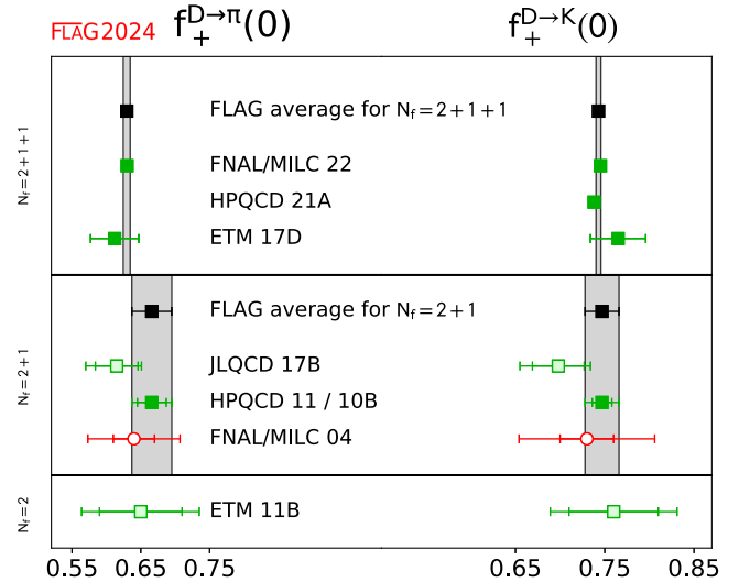
FIG. 17. D \rightarrow \pi \ell \nu and D \rightarrow K \ell \nu semileptonic form factors at q^2 = 0 . The N_f = 2+1 HPQCD result for f_+^{D \rightarrow \pi}(0) is from HPQCD 11, the one for f_+^{D \rightarrow K}(0) represents HPQCD 10B (see Table 29).
