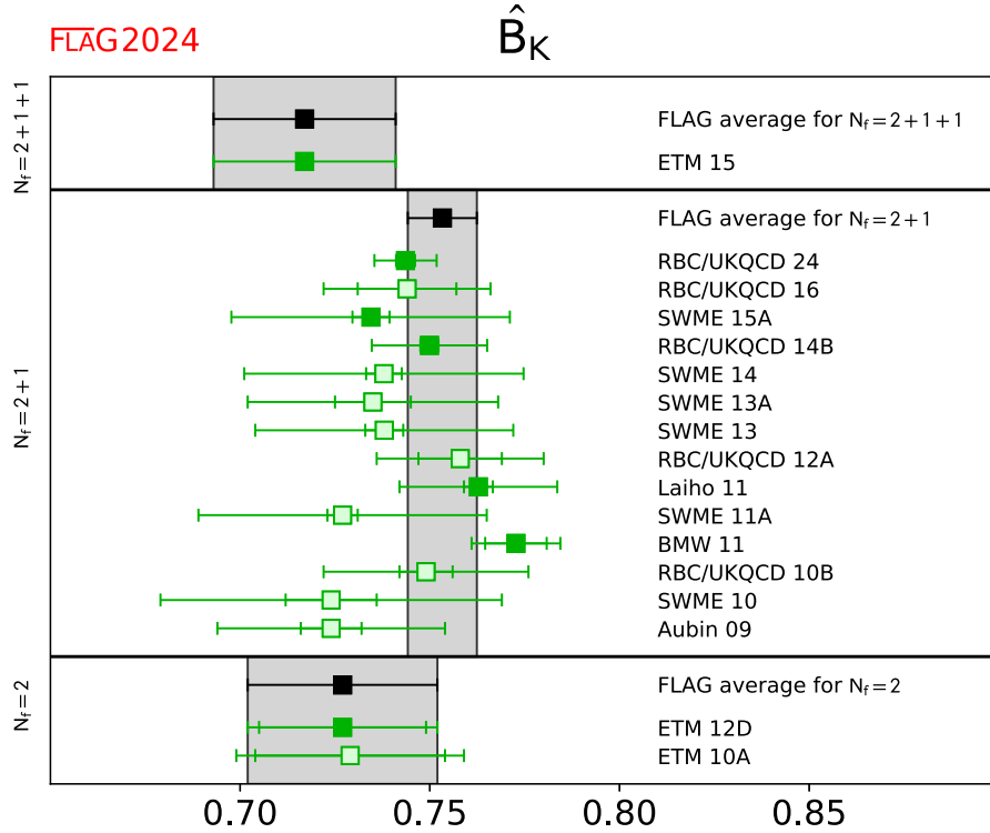
FIG. 14. Unquenched lattice results for the RGI B -parameter \hat{B}_K . The gray bands indicate our averages described in the text. For N_f = 2 + 1 + 1 and N_f = 2 the FLAG averages coincide with the results by ETM 15 and ETM 12D, respectively.
