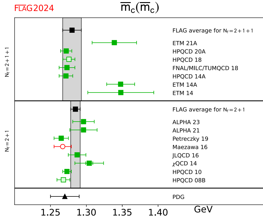
FIG. 5. The charm-quark mass for 2 + 1 and 2 + 1 + 1 flavors. For the latter a large stretching factor is used for the FLAG average due to poor \chi^2 from our fit.
