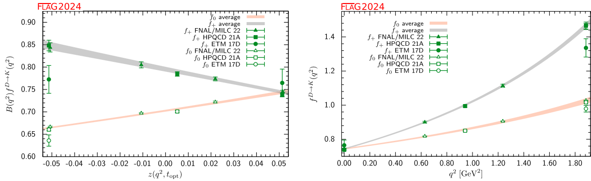
FIG. 18. The form factors f_+(q^2) and f_0(q^2) for D \rightarrow K \ell \nu plotted versus z (left panel) and q^2 (right panel). In the left plot, we removed the Blaschke factors. See text for a discussion of the dataset. The gray and salmon bands display our preferred N^+ = N^0 = 4 BCL fit (seven parameters).
