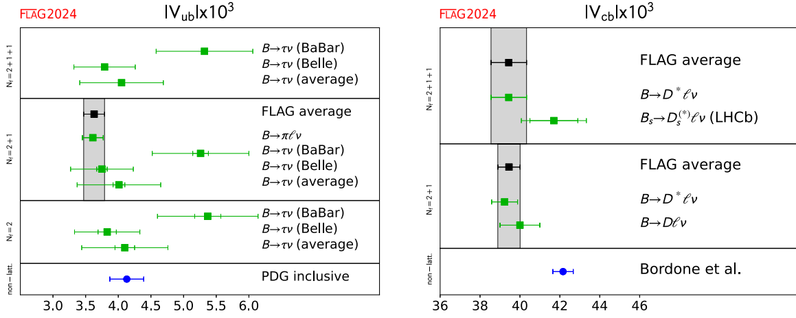
FIG. 35. Left: Summary of |V_{ub}| determined using: (i) the B -meson leptonic decay branching fraction, B(B^- \rightarrow \tau^- \bar{\nu}) , measured at the Belle and BABAR experiments, and our averages for f_B from lattice QCD; and (ii) the various measurements of the B \rightarrow \pi \ell \nu decay rates by Belle and BABAR, and our averages for lattice determinations of the relevant vector form factor f_+(q^2) . The inclusive result is taken from PDG [274]. Right: Same for determinations of |V_{cb}| using semileptonic decays. The inclusive result is taken from Ref. [675].
