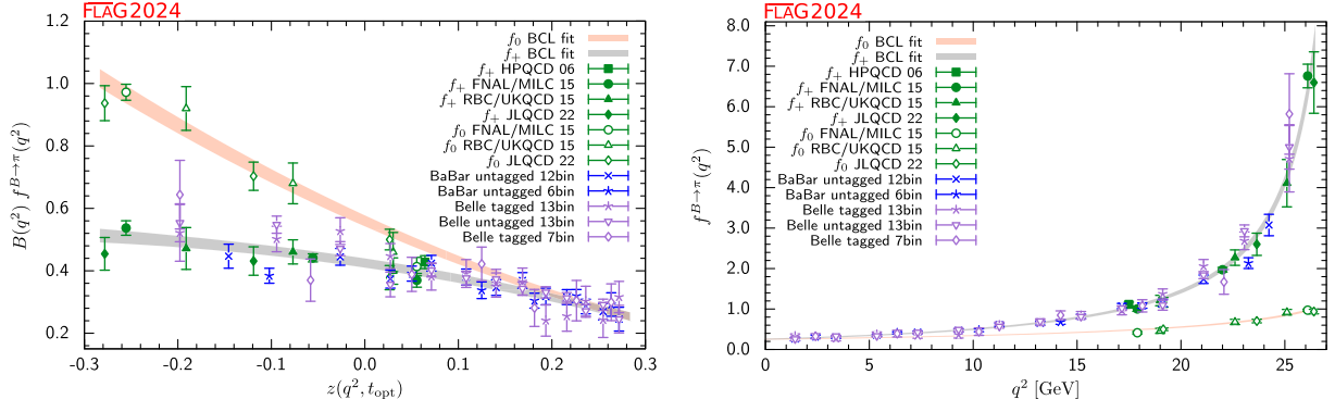
FIG. 31. Lattice and experimental data for f_+^{B \rightarrow \pi}(q^2) and f_0^{B \rightarrow \pi}(q^2) versus z (left panel) and q^2 (right panel). Experimental data has been rescaled by the value for |V_{ub}| found from the joint fit. Green symbols denote lattice-QCD points included in the fit, while blue and indigo points show experimental data divided by the value of |V_{ub}| obtained from the fit. The gray and orange bands display the preferred N^+ = N^0 = 3 BCL fit (five z -parameters and |V_{ub}| ).
