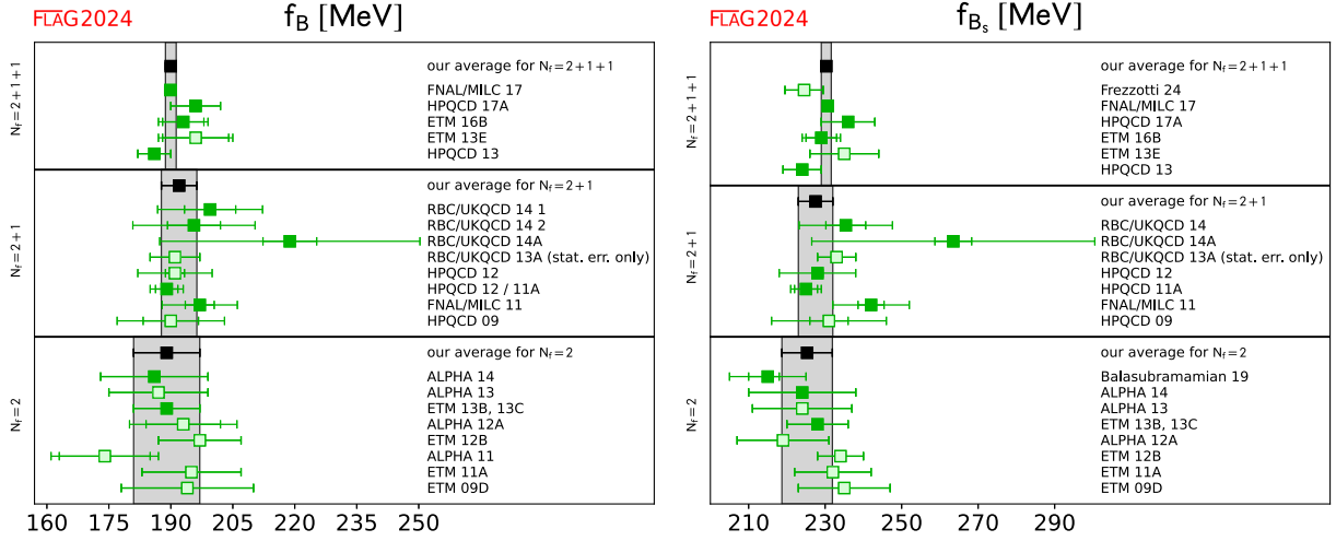
FIG. 21. Decay constants of the B and B_s mesons. The values are taken from Table 33 (the f_B entry for FNAL/MILC 11 represents f_{B^+} ). The significance of the colors is explained in Sec. II. The black squares and gray bands indicate our averages in Eqs. (162), (165), (168), (163), (166) and (169).
