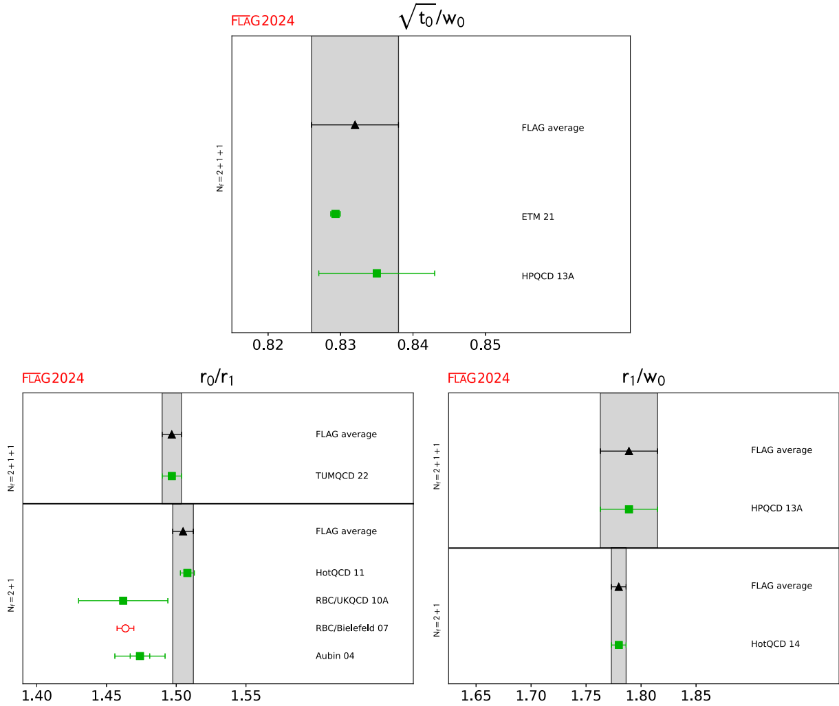
FIG. 53. Results for dimensionless ratios of scales.
