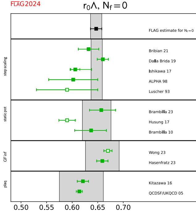
FIG. 39. r_0\Lambda_{\overline{\text{MS}}} estimates for N_f = 0 flavors. As discussed in the text, we group the results by method and estimate pre-ranges. Only full green squares are used in our final ranges, pale green squares indicate that the computations were not published or superseded by later more complete ones.
