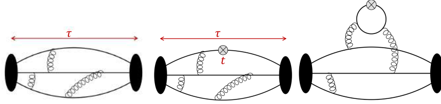
FIG. 41. The two- and three-point correlation functions (illustrated by Feynman diagrams) that need to be calculated to extract the ground-state nucleon matrix elements. Left: the nucleon two-point function. Middle: the connected three-point function with source-sink separation \tau and operator-insertion time slice t . Right: the quark-disconnected three-point function with operator insertion at t .
