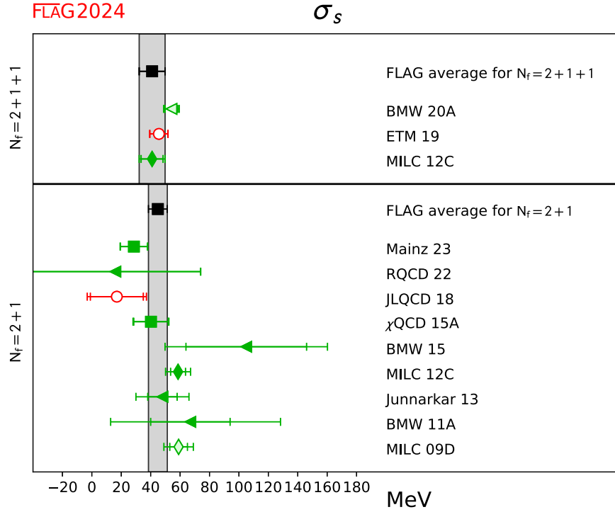
FIG. 47. Lattice results and FLAG averages for \sigma_s for the N_f = 2 + 1 , and 2 + 1 + 1 flavor calculations. Determinations via the direct approach are indicated by squares and circles, the Feynman-Hellmann method by triangles and the hybrid approach by diamonds.
