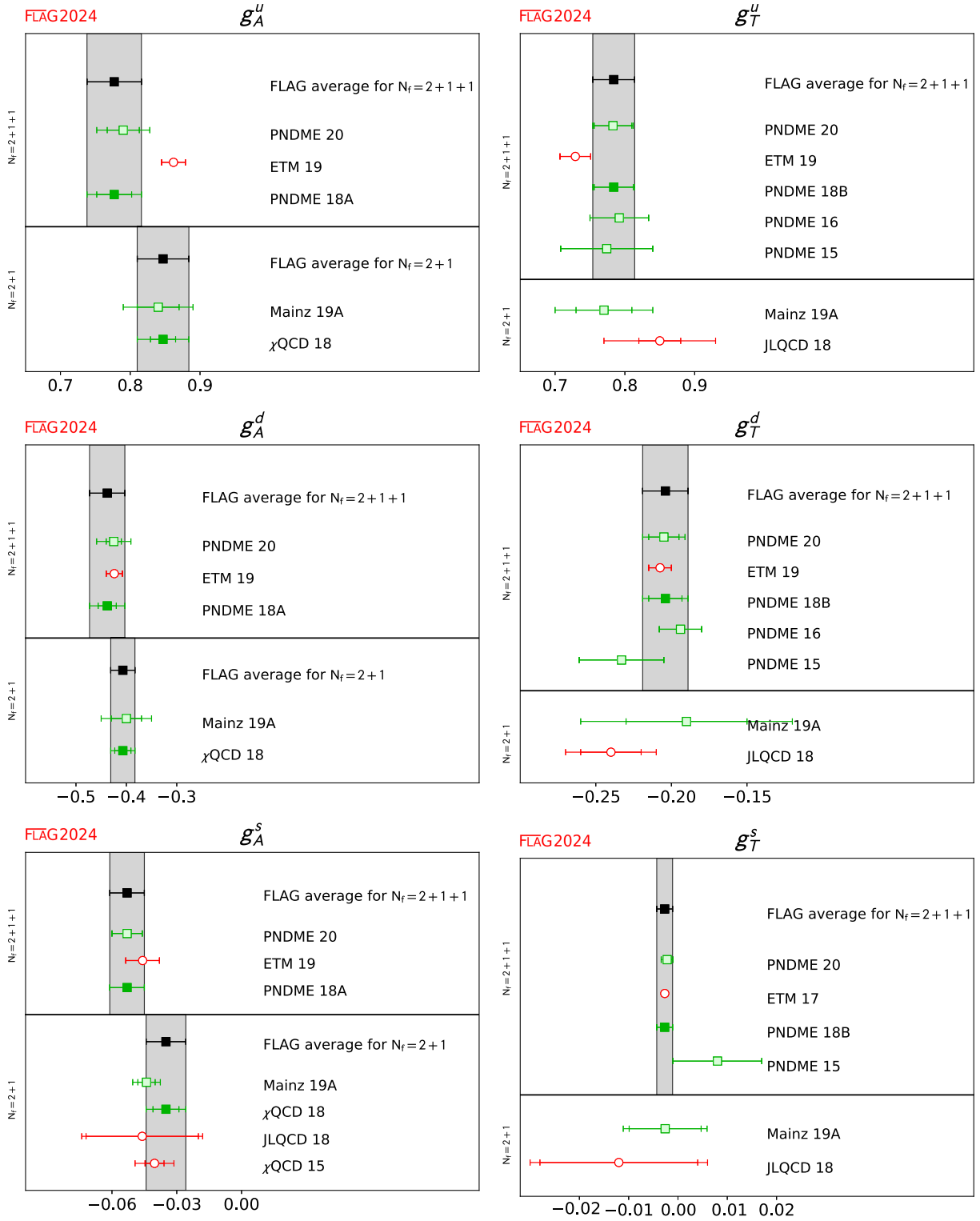
FIG. 45. Lattice results and FLAG averages for g_A^{u,d,s} (left) and g_T^{u,d,s} (right) for the N_f = 2 + 1 and 2 + 1 + 1 -flavor calculations.
