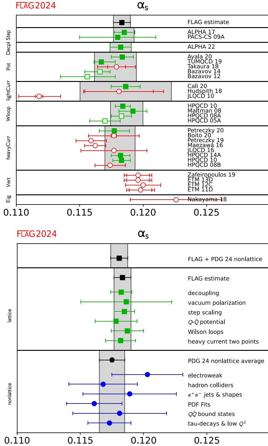
FIG. 40. \alpha_{\overline{\text{MS}}}^{(5)}(M_Z) , the coupling constant in the \overline{\text{MS}} scheme at the Z-boson mass. Top: lattice results, pre-ranges from different calculation methods, and final average. Bottom: Comparison of the lattice pre-ranges and average with the nonlattice ranges and average. The first PDG 24 entry gives the outcome of their analysis excluding lattice results. At the very top we display the weighted average of PDG 24 nonlattice and FLAG lattice estimates, with the error taken from the FLAG estimate (statistics dominated), see Sec. IX J 3.
