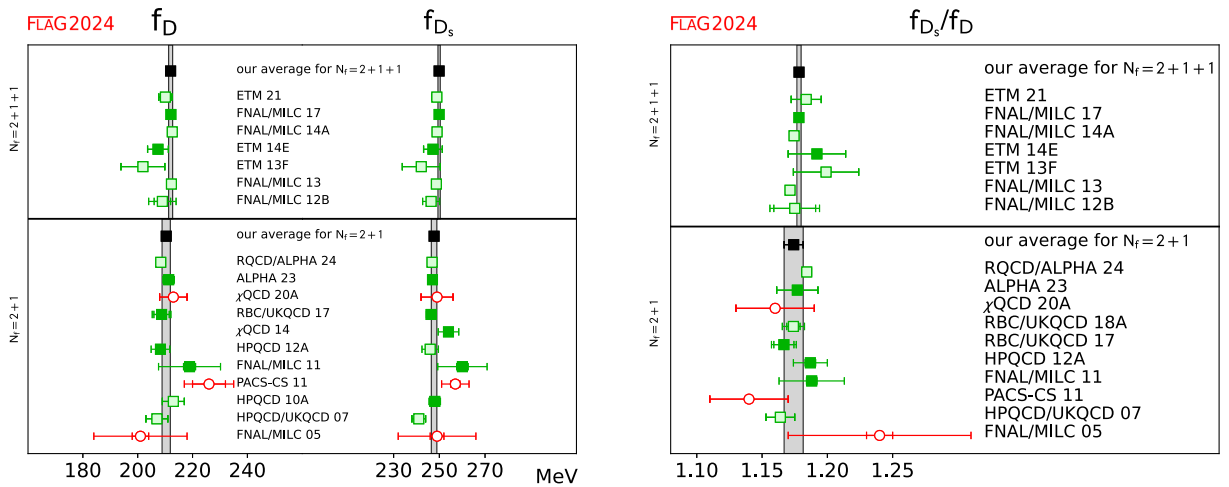
FIG. 16. Decay constants of the D and D_s mesons [values in Table 28 and Eqs. (126)–(131)]. As usual, full green squares are used in the averaging procedure, pale green squares have either been superseded by later determinations or are only published in proceedings or have not been published within the current deadline (April 30, 2024), while empty red circles do not satisfy the criteria. The black squares and grey bands indicate our averages.
