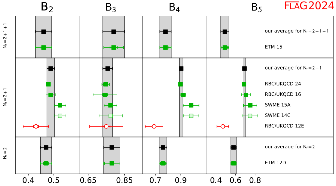
FIG. 15. Results for the BSM B -parameters defined in the \overline{\text{MS}} scheme at a reference scale of 3 GeV (see Table 27).
