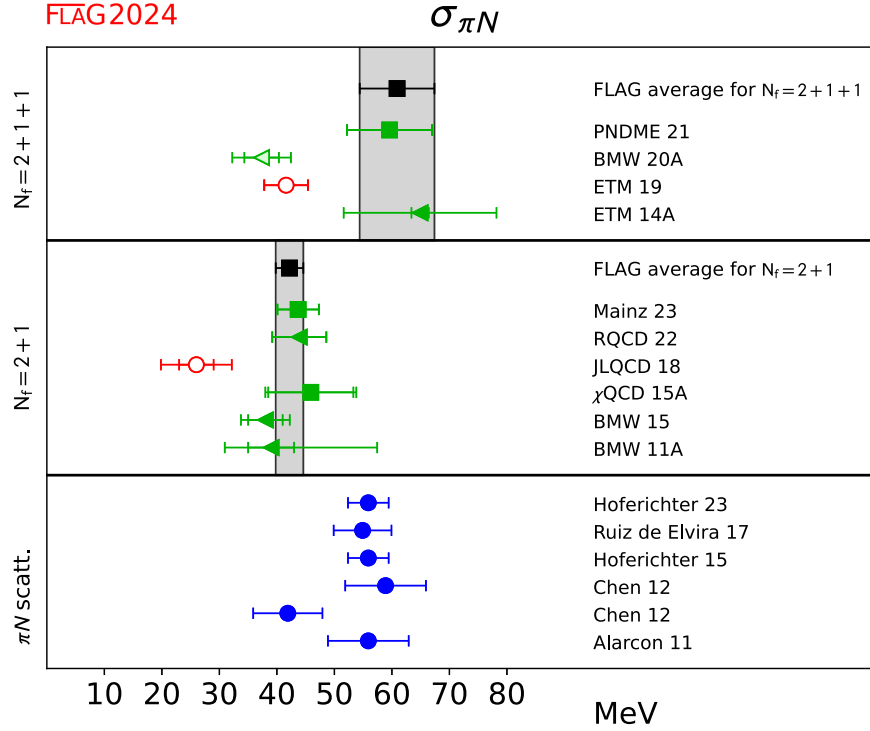
FIG. 46. Lattice results and FLAG averages for the nucleon sigma term, \sigma_{\pi N} , for the N_f = 2 + 1 , and 2 + 1 + 1 flavor calculations. Determinations via the direct approach are indicated by squares and circles, and the Feynman-Hellmann method by triangles. Results from recent analyses of \pi - N scattering [1028–1030,1040,1041] (filled blue circles) are shown for comparison. Note that the charged pion is used to define the isospin limit in these phenomenological analyses, while the neutral pion with M_\pi \sim 135 MeV is usually used to define the physical point in lattice simulations. We adjust the results to be consistent with the latter, applying the correction for the different conventions determined in Ref. [1041].
