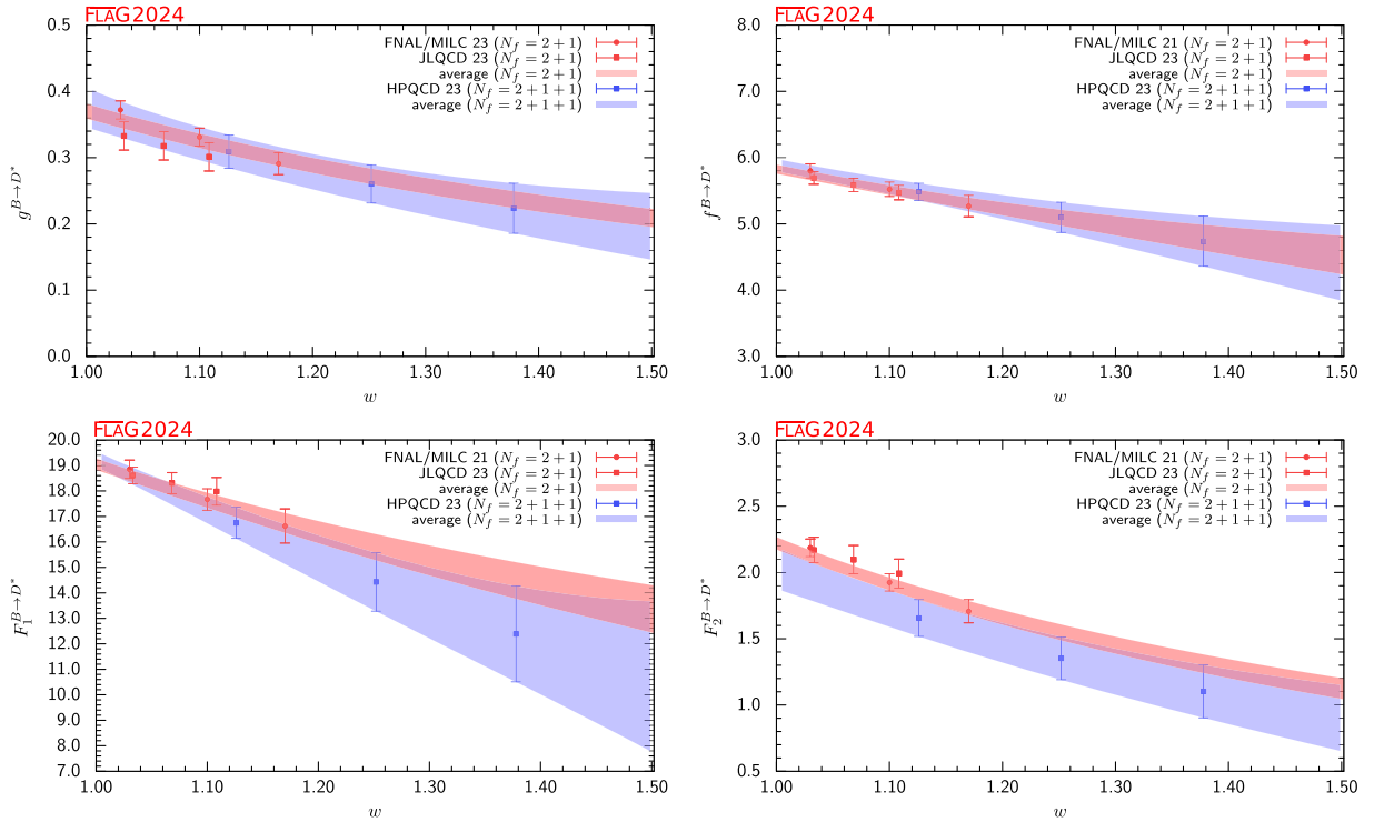
FIG. 29. The form factors g, f, F_1 and F_2 for B \rightarrow D^* \ell \nu as a function of w . The red band displays our preferred (N_g, N_f, N_{F_1}, N_{F_2}) = (2, 3, 3, 2) BGL fit (eight parameters) to N_f = 2 + 1 lattice data. The constraints at zero and maximum recoil are imposed exactly. No use of unitarity constraints and priors has been made. The blue band is obtained using directly the N_f = 2 + 1 + 1 HPQCD 23 [135] results.
