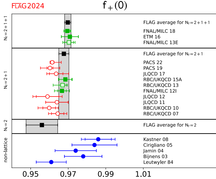
FIG. 8. Comparison of lattice results (squares and empty circles) for f_+(0) with various model estimates based on \chi PT [330,332–335] (filled blue circles). The black squares and gray bands indicate our averages in Eqs. (72) and (73). The significance of the colors is explained in Sec. II.
