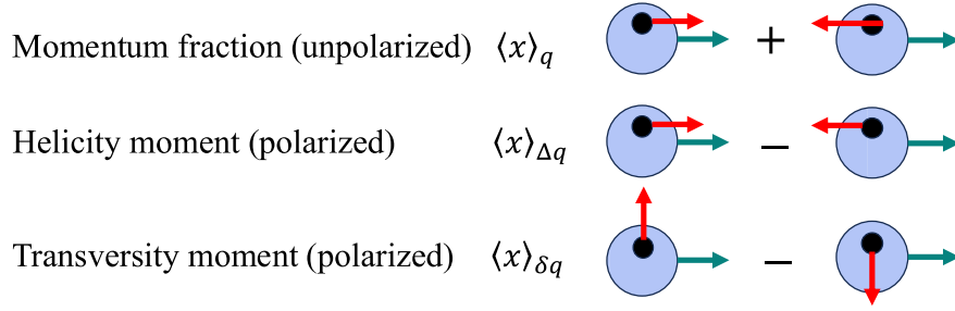
FIG. 48. A pictorial description of the three moments showing the direction of the spin of the quark (red arrow) with respect to the nucleon momentum (green arrow).
