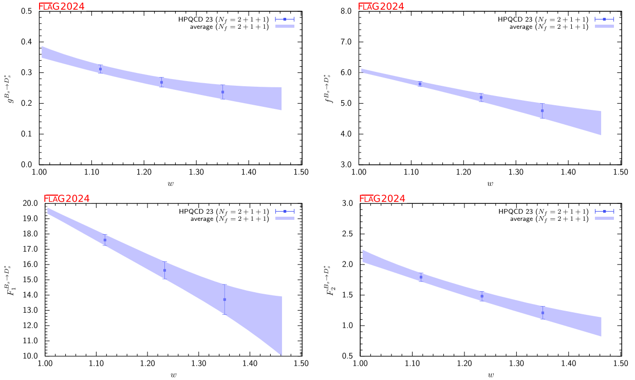
FIG. 30. The form factors g , f , F_1 , and F_2 for B_s \rightarrow D_s^* \ell \nu as a function of w . The blue band is obtained using directly the N_f = 2 + 1 + 1 HPQCD 23 [135] results.
