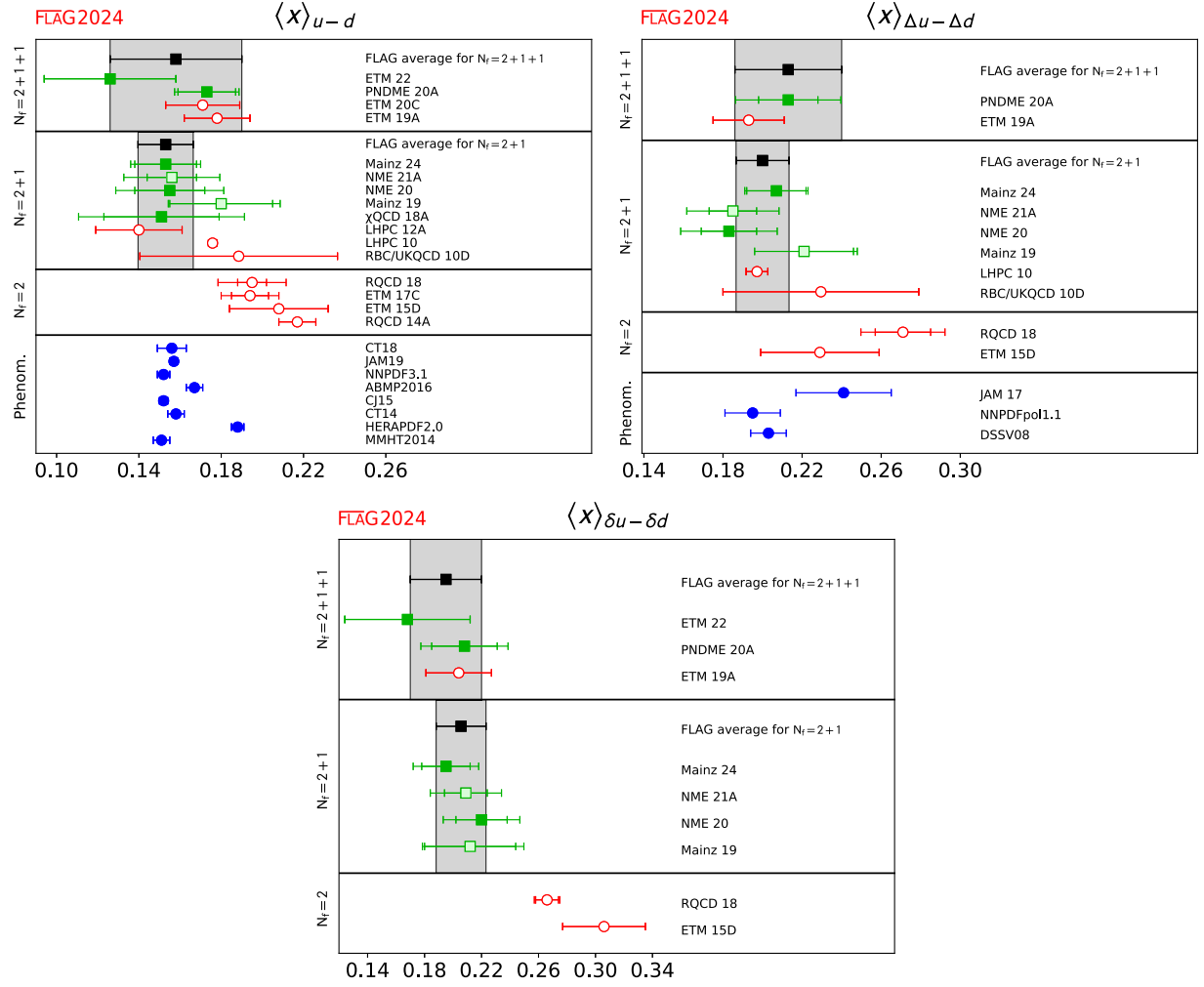
FIG. 49. Lattice-QCD results for the second Mellin moments \langle x \rangle_{u-d} , \langle x \rangle_{\Delta u - \Delta d} and \langle x \rangle_{\delta u - \delta d} . Results from N_f = 2 simulations and publications prior to 2014 have been included as this is the first review of these quantities. For the momentum-fraction and helicity moment, we have also included phenomenological estimates [1048–1058]. For reference, a recent analysis [1059], using a combined set of World DIS data, found \langle x \rangle_{u-d} = 0.143(5) at Q^2 = 4 \text{ GeV}^2 (not shown).
