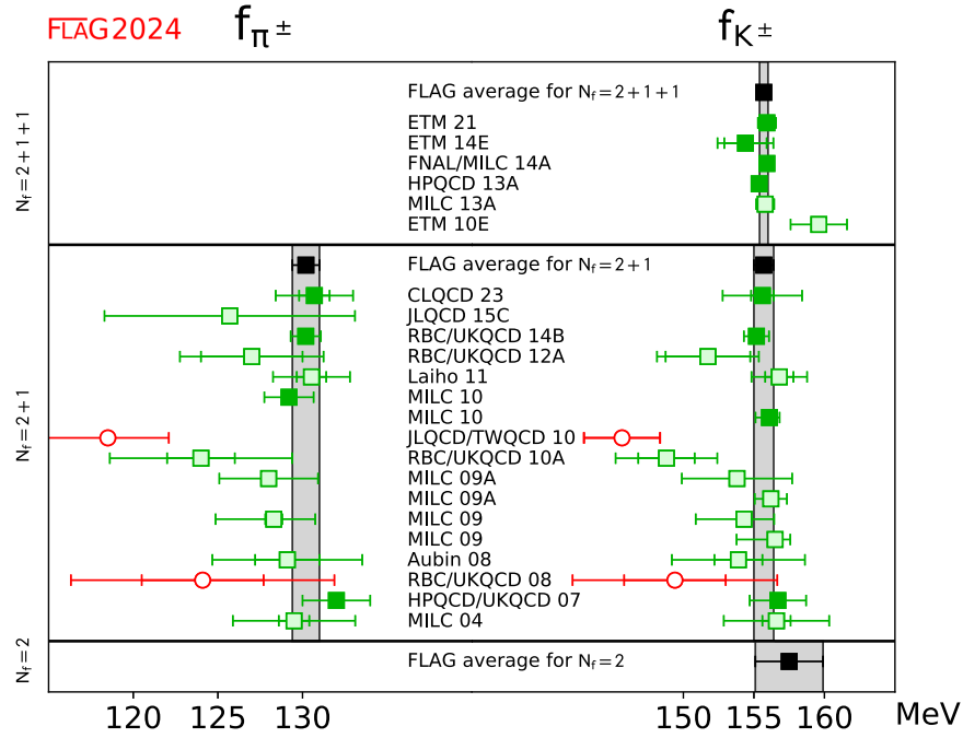
FIG. 13. Values of f_{\pi^\pm} and f_{K^\pm} . The black squares and gray bands indicate our averages in Eqs. (79) and (81).
