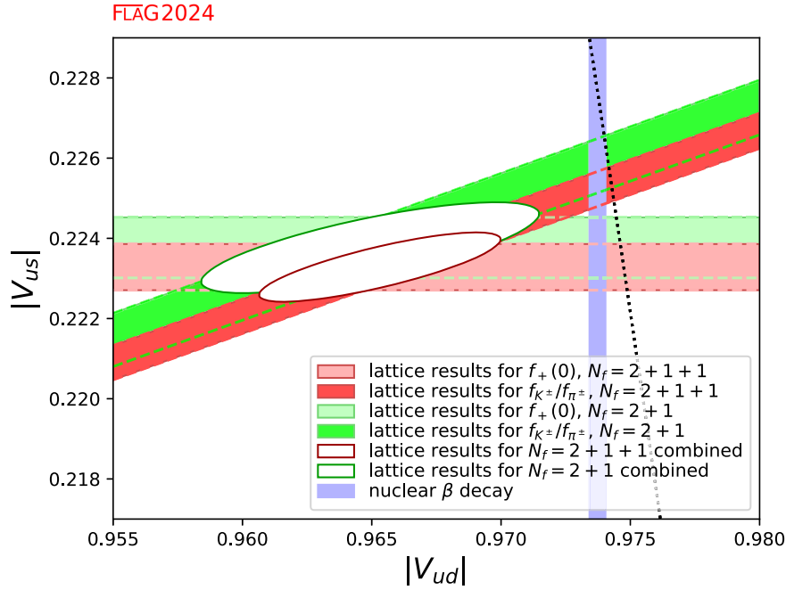
FIG. 11. Same as Fig. 10 but with |V_{us}|/|V_{ud}| obtained using Eq. (68).
