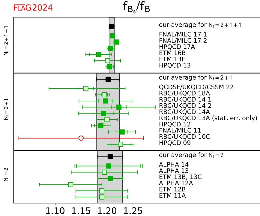
FIG. 22. Ratio of the decay constants of the B and B_s mesons. The values are taken from Table 34. Results labeled as FNAL/MILC 17 1 and FNAL/MILC 17 2 correspond to those for f_{B_s}/f_{B^0} and f_{B_s}/f_{B^+} reported in FNAL/MILC 17. The significance of the colors is explained in Sec. II. The black squares and gray bands indicate our averages in Eqs. (164), (167), and (170).
