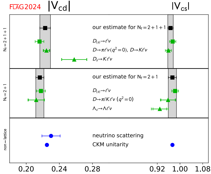
FIG. 20. Comparison of determinations of |V_{cd}| and |V_{cs}| obtained from lattice methods [Eqs. (142), (143), and (145)–(152)] with a nonlattice determination from neutrino scattering (for |V_{cd}| only) [225] and with the Standard Model predictions from a global fit assuming CKM unitarity [396].
