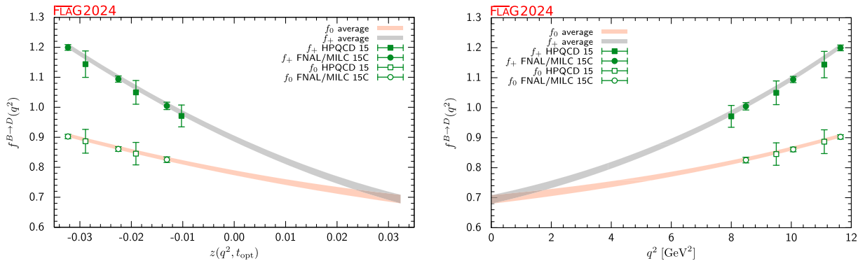
FIG. 28. The form factors f_+(q^2) and f_0(q^2) for B \rightarrow D \ell \nu plotted versus z (left panel) and q^2 (right panel). See text for a discussion of the datasets. The gray and salmon bands display our preferred N^+ = N^0 = 3 BCL fit (five parameters).
