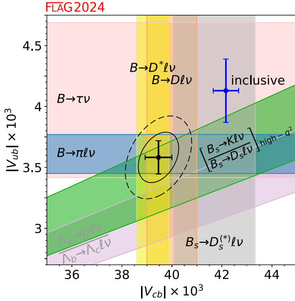
FIG. 36. Summary of |V_{ub}| and |V_{cb}| determinations. The black solid and dashed lines correspond to 68% and 95% confidence-level (C.L.) contours, respectively. The result of the global fit (which does not include |V_{ub}/V_{cb}| from baryon modes nor |V_{cb}| from B_s \rightarrow D_s^{(*)} \ell \nu ) is (|V_{cb}|, |V_{ub}|) = (39.46 \pm 0.53, 3.60 \pm 0.14) \times 10^{-3} with a p -value of 0.66. The lattice and experimental results that contribute to the various contours are the following. B \rightarrow \pi \ell \nu : lattice (FNAL/MILC 15 [124], RBC/UKQCD 15 [125], and JLQCD 22 [126]) and experiment (BABAR [138,139] and Belle [140,141]). B \rightarrow D \ell \nu : lattice (FNAL/MILC 15C [132] and HPQCD 15 [133]) and experiment (BABAR [142] and Belle [143]). B \rightarrow D^* \ell \nu : lattice (FNAL/MILC 21 [136], JLQCD 23 [137], HPQCD 23 [135]) and experiment (Belle [144,145], Belle II [146], HFLAV [148]). B \rightarrow \tau \nu : lattice ( N_f = 2 + 1 + 1 determination of f_B in Eq. (168) [20,36,67,68]) and experiment (BABAR [515] and Belle [514]). B_s \rightarrow K \ell \nu / B_s \rightarrow D_s \ell \nu : lattice (HPQCD 14 [127], RBC/UKQCD 23 [128], FNAL/MILC 19 [592], HPQCD 19 [134]) and experiment (LHCb [676]). \Lambda_b \rightarrow p \ell \nu / \Lambda_b \rightarrow \Lambda_c \ell \nu : lattice (Detmold 15 [499]) and experiment (LHCb [656]). B_s \rightarrow D_s^* \ell \nu / B_s \rightarrow D_s \ell \nu : lattice (HPQCD 19 [134] and HPQCD 19B [646]) and experiment (LHCb [633,634]). The inclusive determinations are taken from Refs. [225,308,675] and read (|V_{cb}|, |V_{ub}|)_{\text{incl}} = (42.16 \pm 0.51, 4.13 \pm 0.26) \times 10^{-3} .
