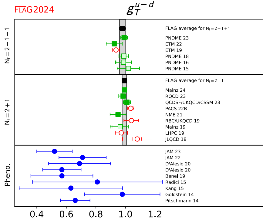
FIG. 44. Lattice results and FLAG averages for the isovector tensor charge g_T^{u-d} for N_f = 2 + 1 and 2 + 1 + 1 flavor calculations. Also shown are phenomenological results using measures of transversity [987,988,1004–1010] (circles). To maintain the independence of lattice QCD and phenomenological results, the JAM22 (private communication supplementing [987]) and JAM23 [988] values shown are those obtained without including input from lattice QCD.
