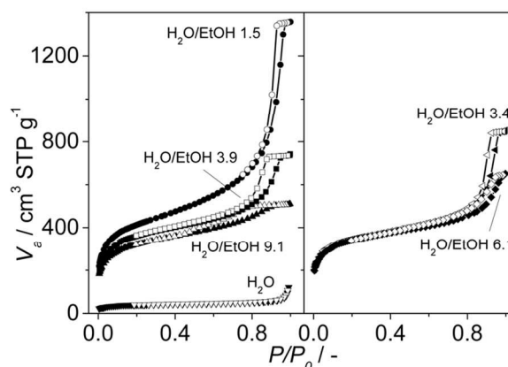
Fig. 7 N 2 adsorption isotherms acquired at 77 K on the samples synthesized at pH 2.5 with different H 2 O/EtOH molar ratios. The H 2 O/EtOH molar ratios used and the topologies obtained were ∞ (MIL-96), 9.1, 6.1 and 3.9 (mixture of MIL-100 and MIL-96), 3.4 (mixture of MIL-100 and MIL-110) and 1.5 (MIL-100), see Table 2. Closed symbols represent adsorption and open symbols desorption branch.
