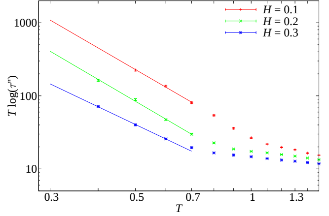
FIG. 12. (Color online) Plot of a lower bound for T \log(\tau) , computed using (35), against T for our three magnetic fields. At very low temperatures this quantity is compatible with a Vogel-Fulcher-Tammann divergence at T = 0 , Eq. (47). Notice the change of regime at around T_c^{\text{high}}(H) (recall Figure 6).
