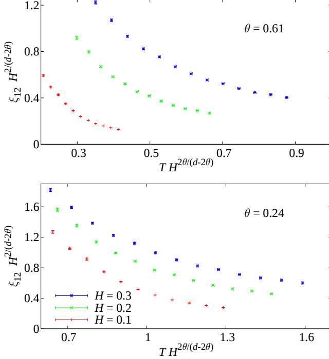
FIG. 17. (Color online) Test of the droplet scaling law, Eq. (23). For each of our magnetic fields, we plot \xi(T, H) H^{2/(d-2\theta)} , as a function of T H^{2\theta/(d-2\theta)} . For a proper choice of the stiffness exponent \theta , data should collapse in a single curve. We try (and fail within the reachable temperature window) to collapse the data with two different estimates of \theta , see Section II C
