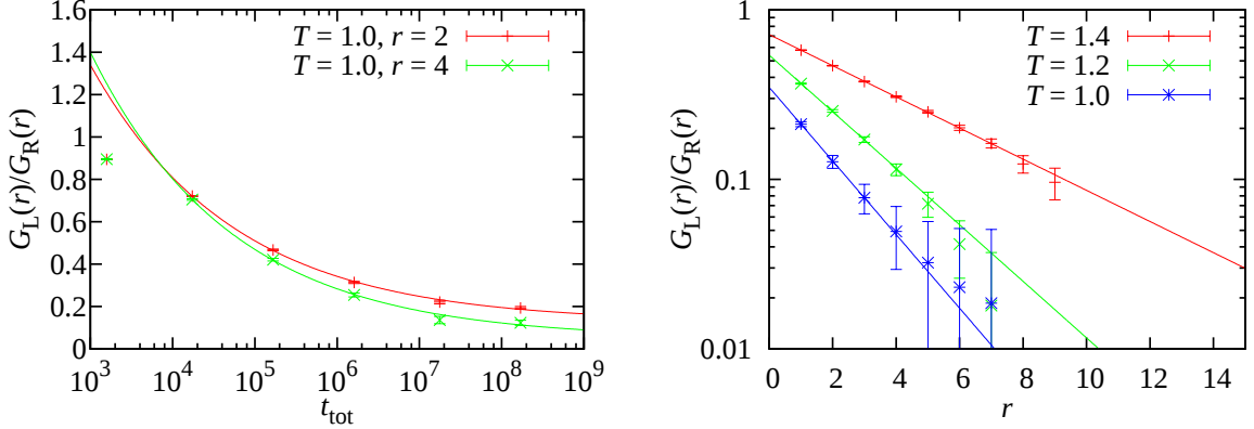
FIG. 23. (Color online) Left : We plot the quotient G_L/G_R for T = 1.0 and H = 0.1 as a function of the total time t_{\text{tot}} for two different values of r . It is clear that even our longest times have small thermalisation effects. The long- t_{\text{tot}} limit may be estimated with a power-law fit (continuous lines). Right : G_L/G_R , extrapolated to infinite t_{\text{tot}} for several temperatures. The curvature observed in Figure 22 has disappeared and a pure exponential decay is now apparent.
