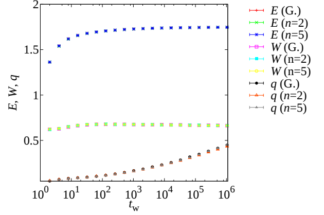
FIG. 18. (Color online) Thermal energy E(t_w) , magnetic energy W(t_w) and overlap q(t_w) as a function of time for L = 8 , T = 0.7 and H = 0.3 . We have plotted the results from a full Gaussian distribution (G.), as well as discretizations with n = 2 and n = 5 . Notice that all three simulations have produced the same equilibrium values for these observables.
