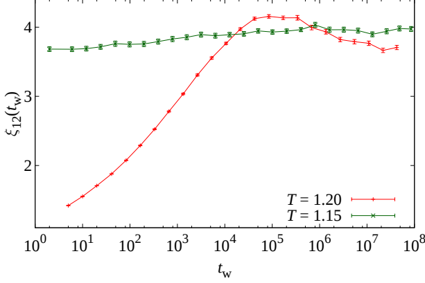
FIG. 20. (Color online) Time evolution of the correlation length \xi_{12} as computed for the replicon correlator for temperatures T = 1.2 and T = 1.15 in our hot annealing, see Section III A. Note that the temperature step T = 1.2 can be regarded as a direct quench, while T = 1.15 already belongs to the annealing part of the run. The maximum for T = 1.2 , where \xi_{12}(t_w) is larger than its equilibrium value, seems to be a generic feature of any direct quench for a spin glass in a field in three dimensions. On the other hand, during the annealing, the time evolution of \xi_{12}(t_w) is monotonic.
