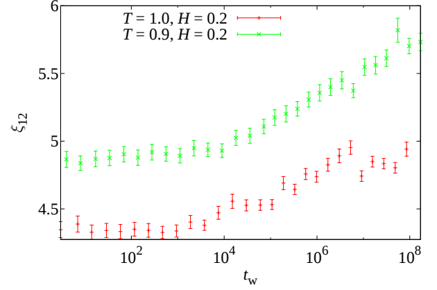
FIG. 14. (Color online) Equilibration of the correlation length: for H = 0.2 , we show the \xi_{12} correlation length as computed from the replicon correlator G_R as a function of t_w . We display data for two constant-temperature steps in the cold annealing (recall that t_w is the time elapsed since the last temperature drop). The constant temperature time step is longer than \tau only for T = 1.0 .
