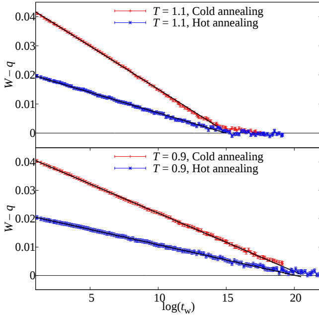
FIG. 5. (Color online) Detail of our two annealing simulations for H = 0.2 at two different temperatures, T = 1.1 and T = 0.9 . We represent the difference W - q as a function of \log(t_w) (we have used \log as the natural logarithm throughout the paper). As pointed out in Figure 3, in this representation W - q is linear for a very long range. More interestingly, if we compute linear fits to (35) (continuous black lines), the intercepts with the horizontal axis are independent of the simulation protocol.
