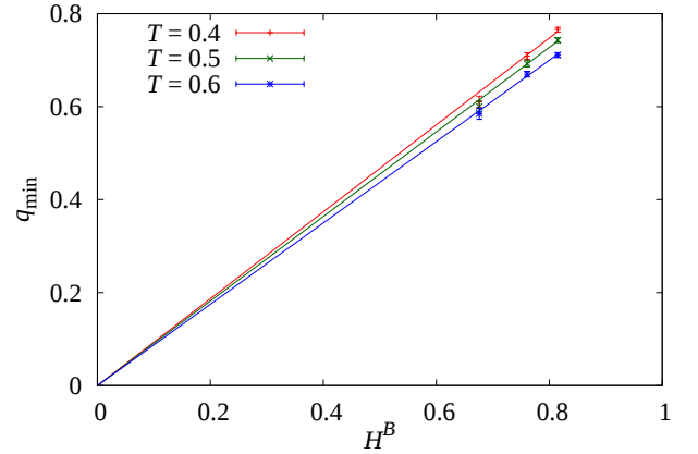
FIG. 9. (Color online) Scaling of the minimum overlap with the magnetic field. A simple power-law behavior, q_{\text{min}} \sim H^B , works well for all our subcritical temperatures, even though we are far from the small- q_{\text{min}} limit.
