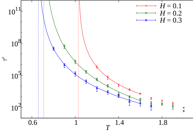
FIG. 6. (Color online) Behavior of the characteristic time \tau' of the stretched exponential (34) as a function of the temperature for the three magnetic fields simulated. We also plot our fits to a power-law divergence of \tau' for a finite temperature, Eq. (36).
