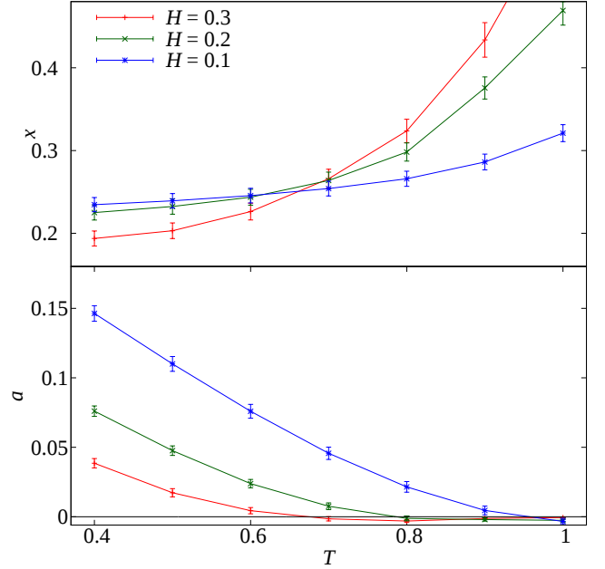
FIG. 7. (Color online) Top : Exponent x of the extrapolation of the difference between W(t_{\text{tot}}) and q(t_{\text{tot}}) , Eq. (39), as a function of temperature, for our three external magnetic fields. Value computed from three-parameter fits. Bottom : As above, for the asymptote a .
