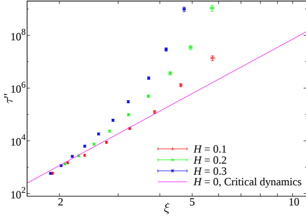
FIG. 15. (Color online) Logarithmic plot of \tau'' , computed in Section III, versus the correlation length ( \xi_{12} ) for the three magnetic fields simulated. Data are in equilibrium. For comparison, we also show the critical dynamics for H = 0 , \tau \sim \xi^z , with z = 6.86 [20].
