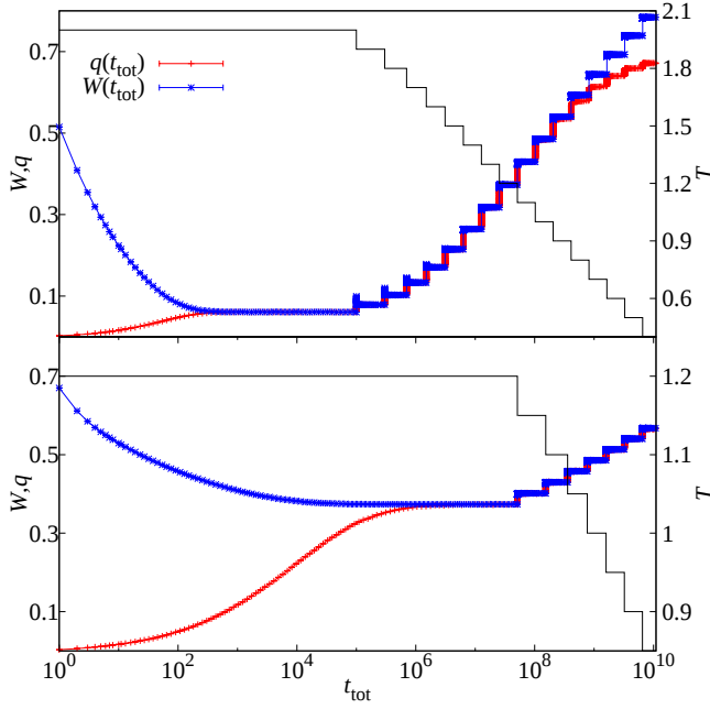
FIG. 1. (Color online) Overview of our two annealing simulations for H = 0.2 . We show the evolution of q(t_{\text{tot}}) [the red (lower) curve] and W(t_{\text{tot}}) [the blue (upper) curve] during the whole simulation. The continuous black line indicates the temperature throughout the simulation (see right-hand vertical axis for the scale). The top panel corresponds to the cold annealing and the bottom panel to the hot annealing (see Table II). Notice how, in the former, the system is not able to reach equilibrium for the lowest temperatures (as signaled by different values of W and q at the end of each temperature step).
