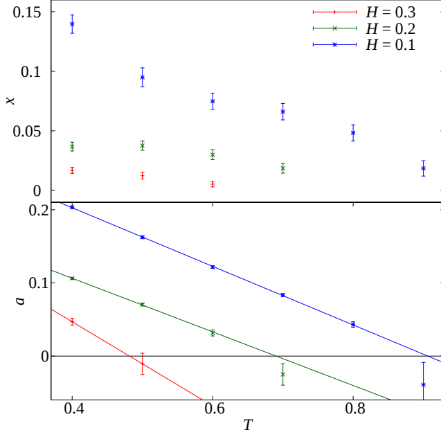
FIG. 10. (Color online) Top : Exponent x of the extrapolation of the difference between W(t_w) and q(t_w) , Eq. (44), as a function of temperature, for our three external magnetic fields. Values computed in a three-parameter fit. Bottom : As above, for the asymptote a . Lines are linear fits to the points where a(T, H) > 0 (for H = 0.3 we included as well T = 0.5 in the fit).
