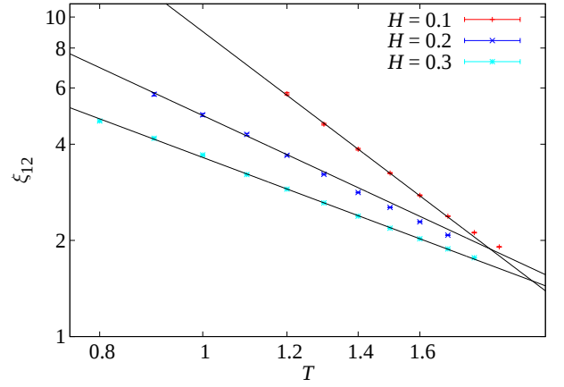
FIG. 16. (Color online) Logarithmic plot of the equilibrium correlation length \xi_{12} versus the temperature for the three magnetic fields simulated. Lines are fits to \xi_{12}(T) = a_H / T^{b_H} , see Eq. (48). When assessing the high-temperature data for H = 0.1 , recall that the critical temperature without a field is T_c^{H=0} = 1.1019(29) [82].
