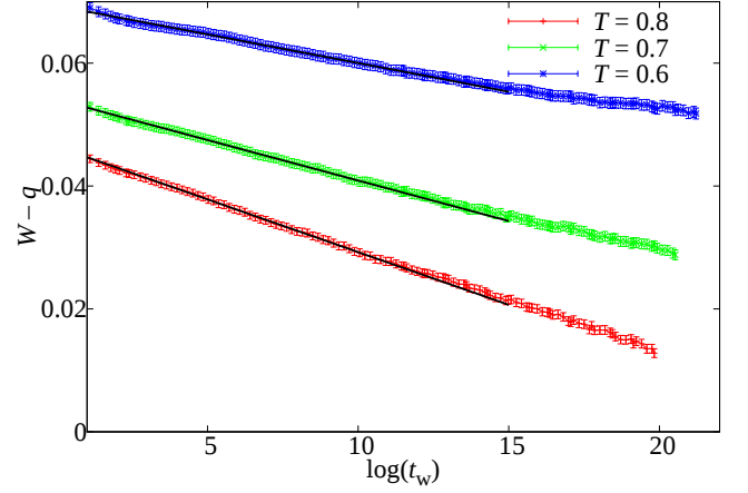
FIG. 11. (Color online) W - q as a function of \log(t_w) for several low temperatures and H = 0.2 . Even in this temperature range we can identify a wide linear regime.
