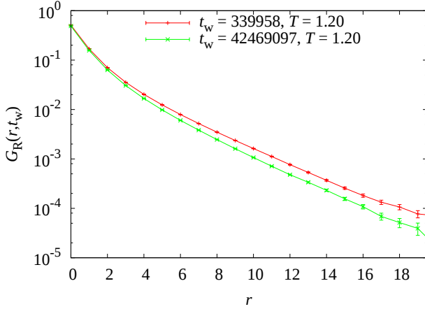
FIG. 21. (Color online) Comparison of the non-equilibrium correlator G_R(r; t_w) with the corresponding equilibrium value for the initial temperature, T = 1.2 , in our hot annealing (i.e., in a direct quench run). The time t_w corresponds to the maximum correlation length in Figure 20.
