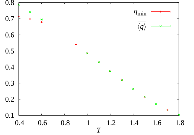
FIG. 8. (Color online) Extrapolations to infinite time of W(t_{\text{tot}}) \rightarrow \overline{q} and q(t_{\text{tot}}) \rightarrow q_{\text{min}} for H = 0.2 , according to (42). We use the same exponent x computed in Figure 7.
