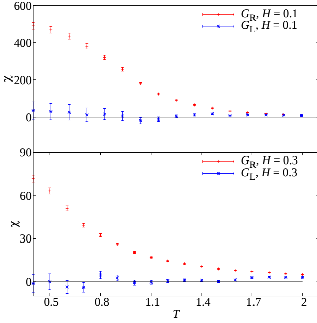
FIG. 13. (Color online) Replicon and longitudinal susceptibilities in our cold annealings for H = 0.1, 0.3 (we plot the last t_w for each T ). The plot contains both equilibrium and non-equilibrium data.
