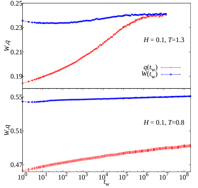
FIG. 2. (Color online) Detail of our annealing simulation for H = 0.1 at two different temperatures, T = 1.3 and T = 0.8 . Notice how in the second case, despite the longer simulation time, the system does not reach equilibrium.
