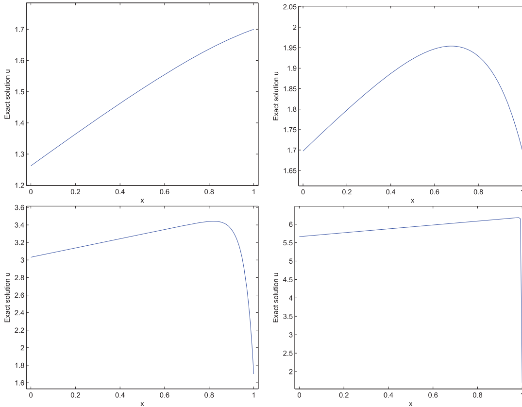
Figure 1. Exact solution for b \equiv 1.9 , c \equiv 0 , f \equiv 1 , \alpha_0 = 1/(\delta - 1) , \alpha_1 = 0 , \gamma_0 = 0.4 and \gamma_1 = 1.7 , with \delta = 1.6 (1st row, left), \delta = 1.4 (1st row, right), \delta = 1.2 (2nd row, left) and \delta = 1.1 (2nd row, right), showing development of a boundary layer when \delta is near 1.
