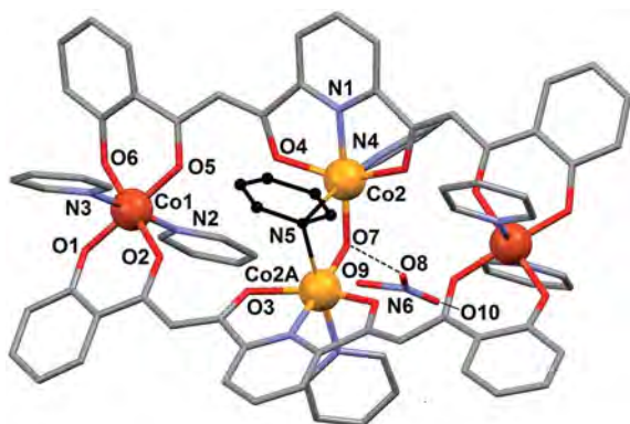
Fig. 3 Molecular structure of [Co 4 (L) 2 (OH)(py) 7 NO 3 ( 1 ) with crystallographically unique heteroatoms labelled. The carbon atoms are in grey except these of the central μ-pyridine group, which have been emphasized in black. The hydrogen atoms are not shown. Only one of two disordered positions of NO 3 - and μ-pyridine are shown.
