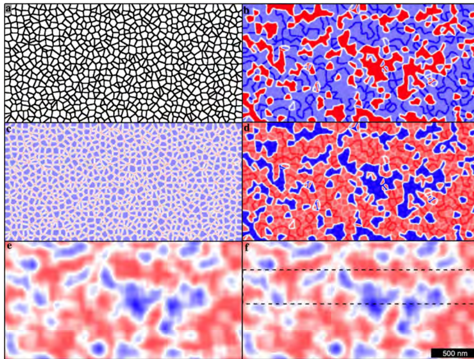
Fig. A1. (a) Representative model nanostructure of the coarse CZ created by eroding Voronoi cells constructed upon a constrained random distribution of points. (b, c) y and z components of the magnetisation respectively. The island easy axis distribution is based on an equally populated random distribution, modified by the magnetisation of neighbouring islands to introduce a degree of clustering. (d) XPEEM signal generated by projecting the magnetisation components onto the X-ray direction. The in-plane component of this direction is parallel to the y direction of the simulation cell, and is 16^\circ out-of-plane. (e) XPEEM signal after having been blurred by a square 120\text{ nm} \times 120\text{ nm} convolution kernel. (f) XPEEM signal after having been down sampled so each pixel is 10\text{ nm} and random noise added, so the experimental and simulated images could be compared. The dashed box represents the area in Fig. 5a.
