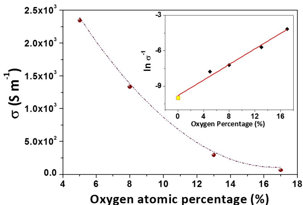
Figure 4. Electrical conductivity as a function of oxygen content ( C_O = 5, 8, 13, and 17%). The line is a guide to the eye. Inset: Fit (solid line) to the experimental data (full diamonds) using the expression for carrier concentration for an intrinsic semiconductor.
