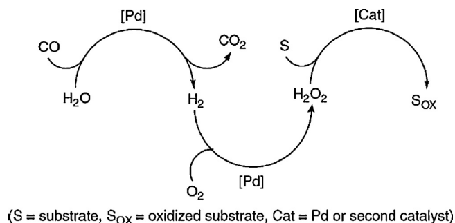
Fig. 7. The mechanism for the selective oxidation of lower alkanes with in-situ generated \text{H}_2\text{O}_2 . Reprinted with permission from [73].
