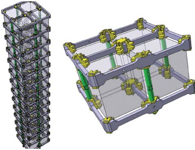
Fig. 1 Left one of the 19 CUORE towers. Right a 4-crystal plane. Two copper frames ( grey ) joined by four columns ( green ) form the mechanical structure that secures four crystals by means of polytetrafluoroethylen (PTFE) supports ( yellow )
