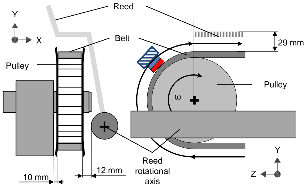
Fig. 5.5: Relevant distances of components on the left side of the demonstrator
