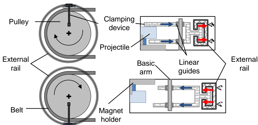
Fig. 8.5: Mobile clamping part with external rail as fixed guiding element
