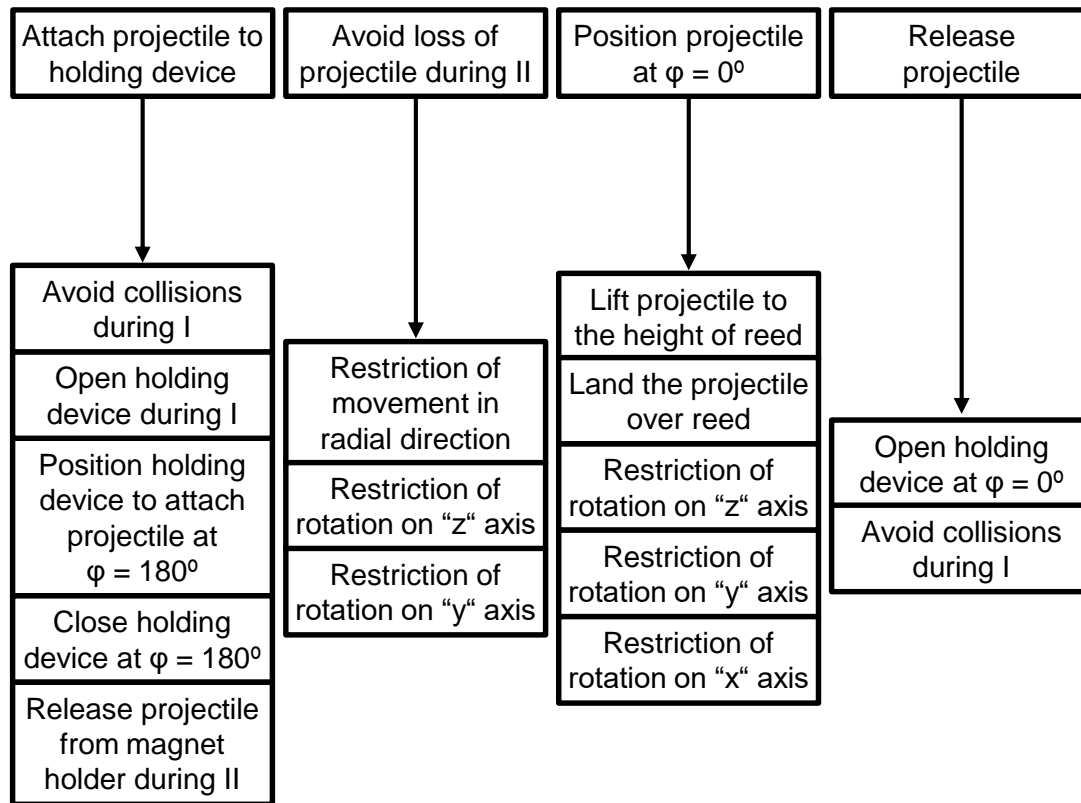
Fig. 6.7: Final functional structure of the left side
