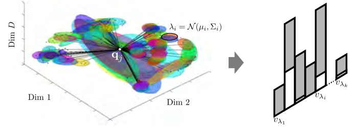
Fig. 2. GMM representation and Soft-assignment-BoF. Grey bars represents the BoF while white highlighted bars represents the \mathbf{q}_j sample contribution.
