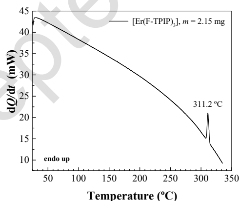
Figure 3. DSC curve of [\text{Er}(\text{F-TPIP})_3] complex
