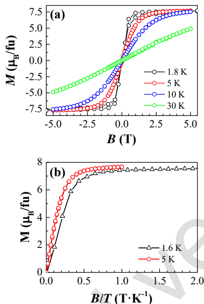
Figure 6. (a) Hysteresis loops at different temperatures for [\text{Er}(\text{F-TPIP})_3] with a sweeping rate of 90 \text{ Oe s}^{-1} ; (b) reduced magnetization plots for [\text{Er}(\text{F-TPIP})_3] at 1.6 and 5 K.
