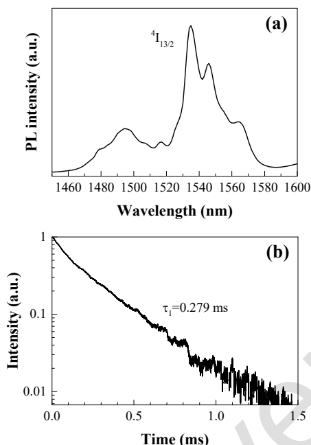
Figure 4. (a) PL spectrum and (b) luminescence decay profile of [\text{Er}(\text{F-TPIP})_3] in powder form.
