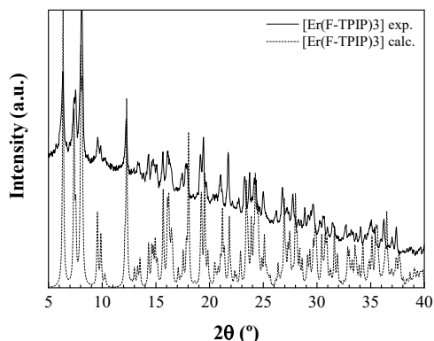
Figure 2. Experimental versus calculated X-ray powder patterns for [\text{Er}(\text{F-TPIP})_3]
