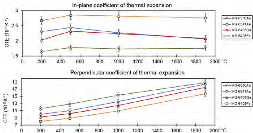
Fig. 12. Secant coefficients of thermal expansion 20–200 °C, 20–500 °C, 20–1000 °C and 20–1900 °C. The values shown are taken from the cooling-down ramp of the measurement. (A colour version of this figure can be viewed online.)
