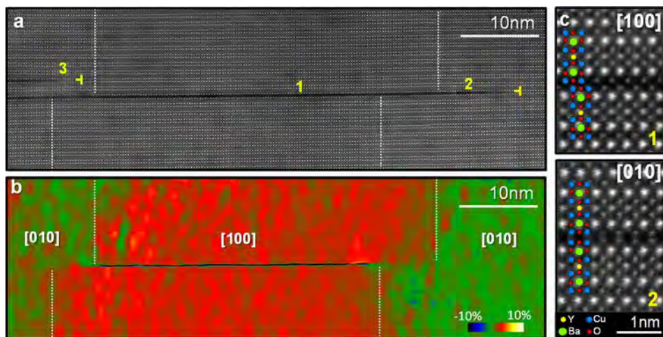
FIG. 3. (a) A composition of consecutive atomic resolution Z-contrast images along a particular Y248 planar defect of a YBCO nanocomposite cross-sectional specimen. (b) e_{xx} deformation map showing in colors (red and green) different deformation values. Region 3 in (a) was taken as a reference area. (c) Close up views of regions 1 and 2 labeled in (a) corresponding to two sides of a twin boundary, which permits determination of the [010] and [100] zone axes in (b). The brightest spots correspond to Ba columns, followed by Y and finally by Cu, being the darkest contrast shown by the atomic planes containing Cu-O chains.
