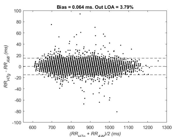
Figure 2. Bland–Altman plot: RR_{H7g} vs. RR_{AW} . Mean of the difference of the RR series \pm 2 *std values (limits of agreement, LOA).
