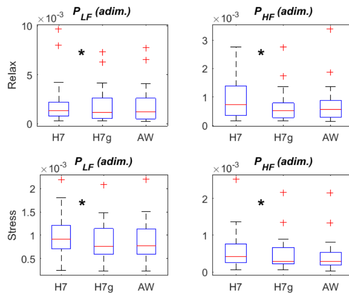
Figure 4. HRV parameters: frequency domain, derived from RR_{H7} , RR_{H7g} and RR_{AW} . * denotes significant differences ( p < 0.05 ) between adjacent boxplots. Adim refers to adimensional units.
