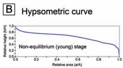
Fig. 3. A) Licus Vallis basin and stream ordering according to Strahler's classification. 1: Impact crater with a possible paleolake that eventually overflowed; 2: Channel interrupted by impact craters. B) Hypsometric curve of the basin. C) Smoothened profile of the main channel. See color figure in the web.
