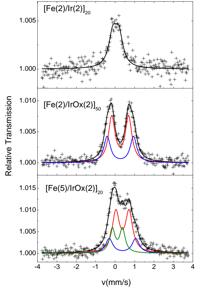
FIG. 10. Mössbauer spectra measured at room temperature. Each panel shows the experimental spectra (+), the overall fit (solid black lines), and the different components: 1 (red), 2 (blue), and 3 (olive) used to fit the experimental spectra.
