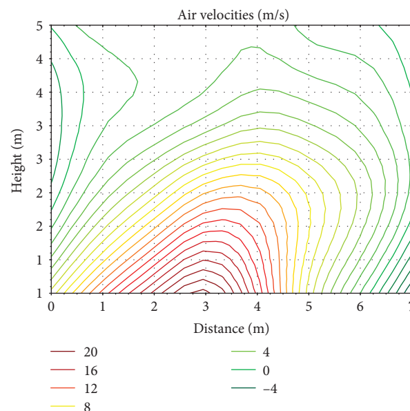
FIGURE 9: Magnitude of air velocity at the plane of the back fan of the sprayer from 3D anemometer measurements, obtained with the sprayer in a low gear and with a blade setting of 4.5.
