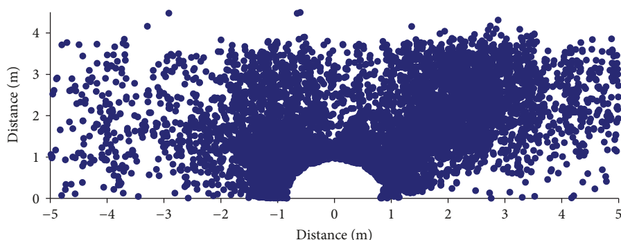
FIGURE 10: Droplets detected by the laser scanner in the plane of the back fan of the sprayer functioning in a low gear and with a blade setting of 4.5.
