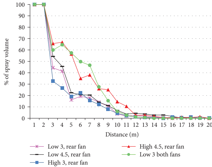
FIGURE 4: Percentage of spray volume detected by the laser within circular crowns of 1 m width for five air flow regulation settings.
