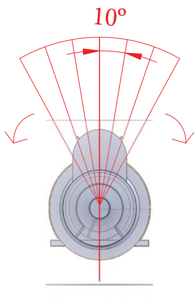
FIGURE 6: Angular sectors used in the analysis of spray direction.
