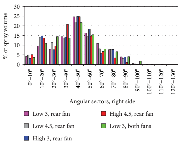
FIGURE 7: Percentage of spray volume for each angular sector for the right side of the sprayer.
