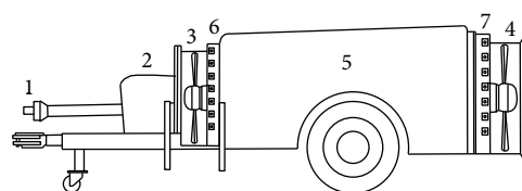
FIGURE 1: Air-assisted sprayer equipped with two reversed-rotation axial fans (1: PTO; 2: pump; 3: front fan; 4: rear fan; 5: tank; 6: front nozzles; 7: rear nozzles).
