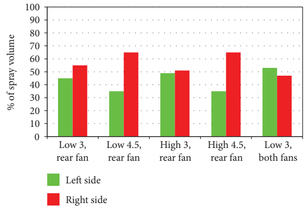
FIGURE 5: Percentage of spray volume detected by the laser on the right and left sides of the sprayer.
