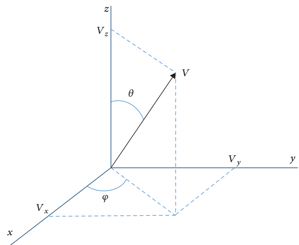
FIGURE 3: Polar coordinates versus Cartesian coordinates.
