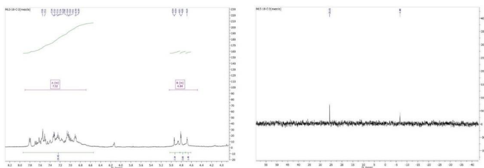
Figura 12. Espectros ^1\text{H} , ^{31}\text{P}\{^1\text{H}\} RMN de [\text{Au}(\text{CL-2a})\text{PPh}_3] (5)
