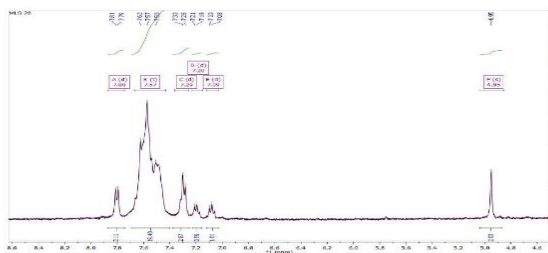
Figura 14. Espectro ^1\text{H} -RMN de [\text{Au}(\text{CL-2a})\text{PPh}_3] (5)
