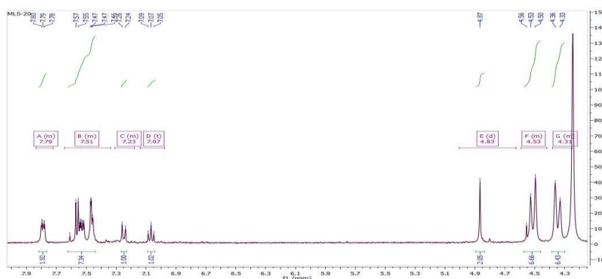
Figura 11. Espectro ^1\text{H} -RMN de [\text{Au}(\text{CL-2a})\text{PTA}] (1)
