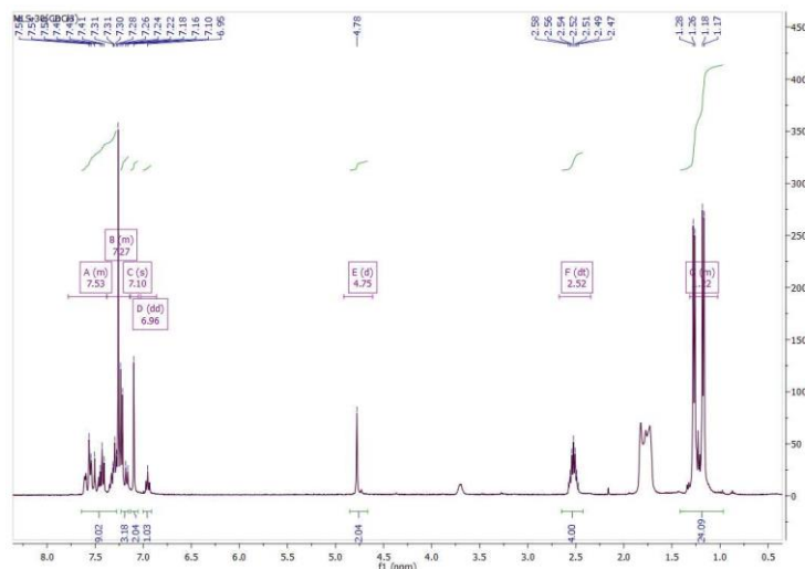
Figura 15. Espectro ^1\text{H} -RMN de [\text{Au}(\text{CL-2a})\text{IPr}] ( 7 )
