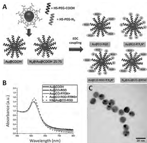
Fig. 1 Functionalization and characterization of AuNPs. (A) Scheme of the stabilization of gold nanoparticles synthesized by reduction with sodium citrate with either one or two different pegylated chains and further functionalization by EDC coupling reaction with (2-aminoethyl) trimethylammonium hydrochloride (R 3 N + ) and/or RGD. Characterization of the AuNPs by (B) UV-Vis spectroscopy and (C) TEM.
