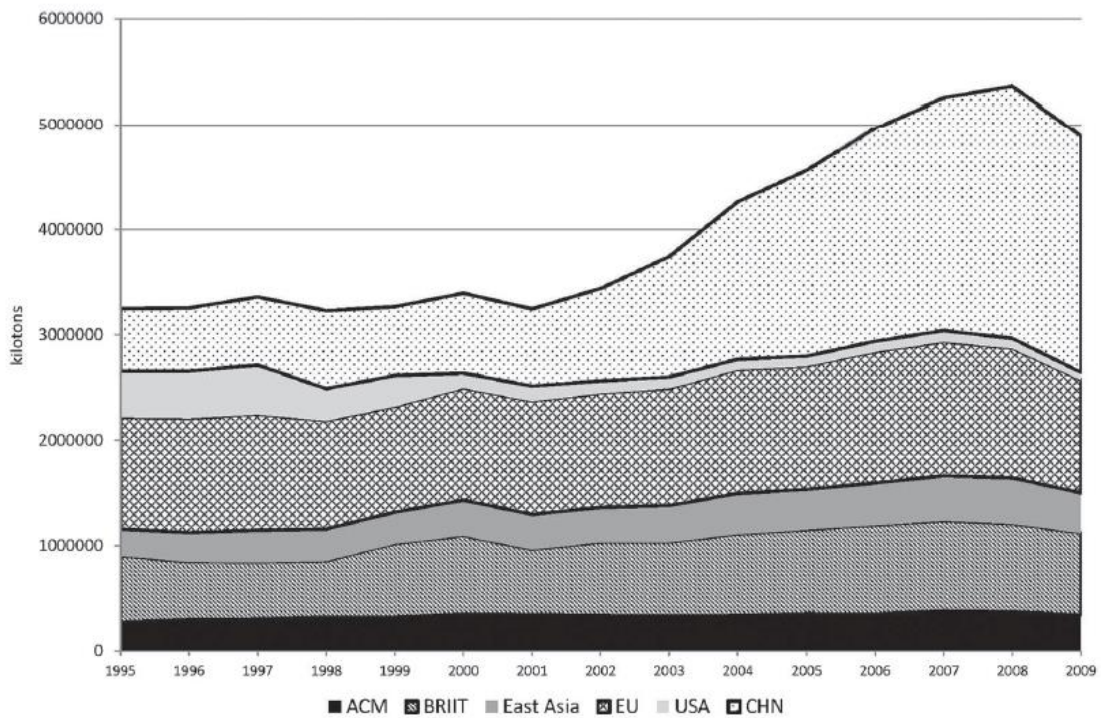
Figura 6. CO2 emissions embodied in exports by world regions, 1995-2009.
